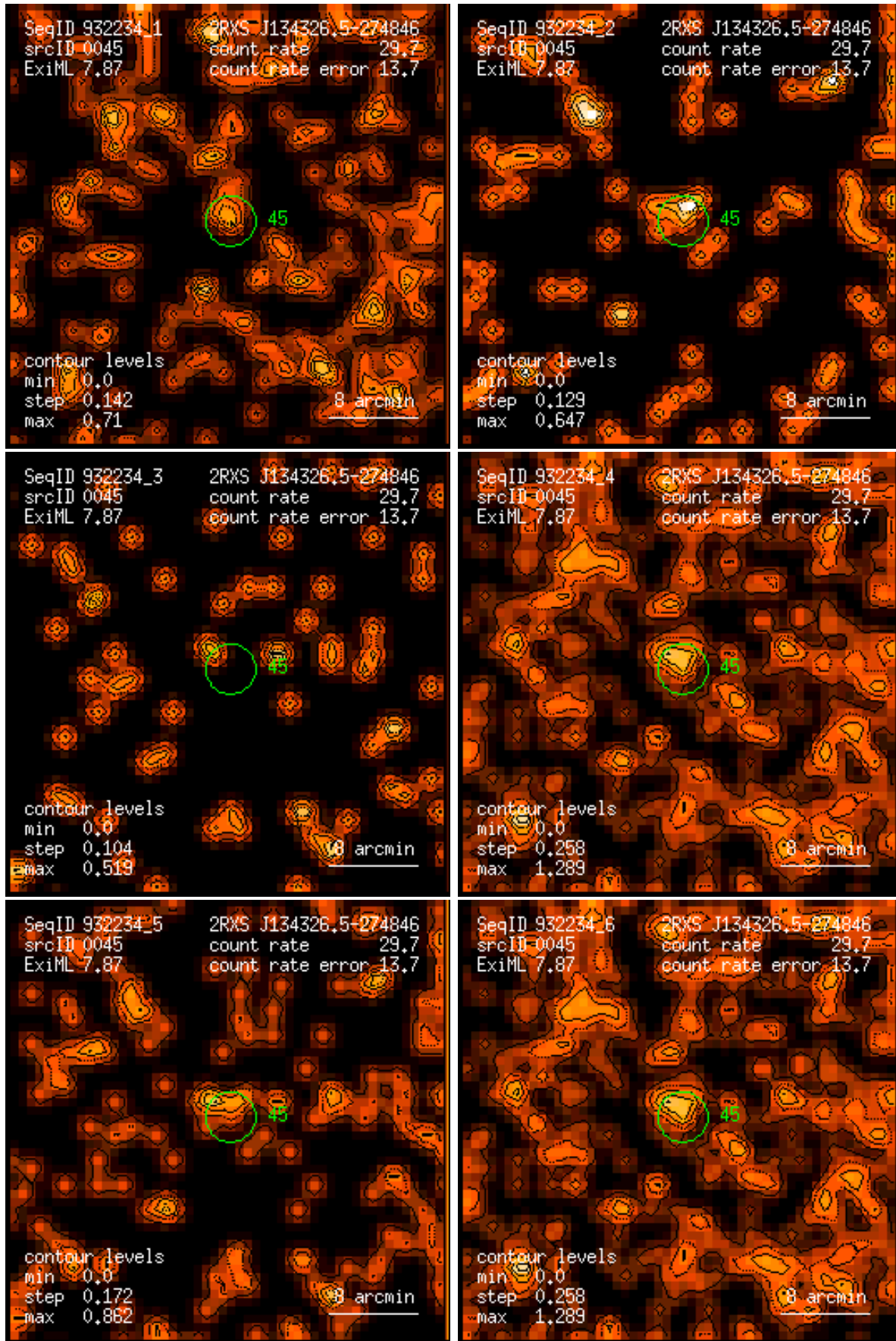
Figure 45: RASS 932234: detection 0045: band rate images, Gaussian filter: (1) PSPC channels 11 – 41, (2) 52 – 90, (3) 91 – 201, (4) 11 – 235, (5) 52 – 201, (6) 11 – 201. Broad band rates in counts/ks. Band rate contour levels in counts/ks/arcmin 2 .
