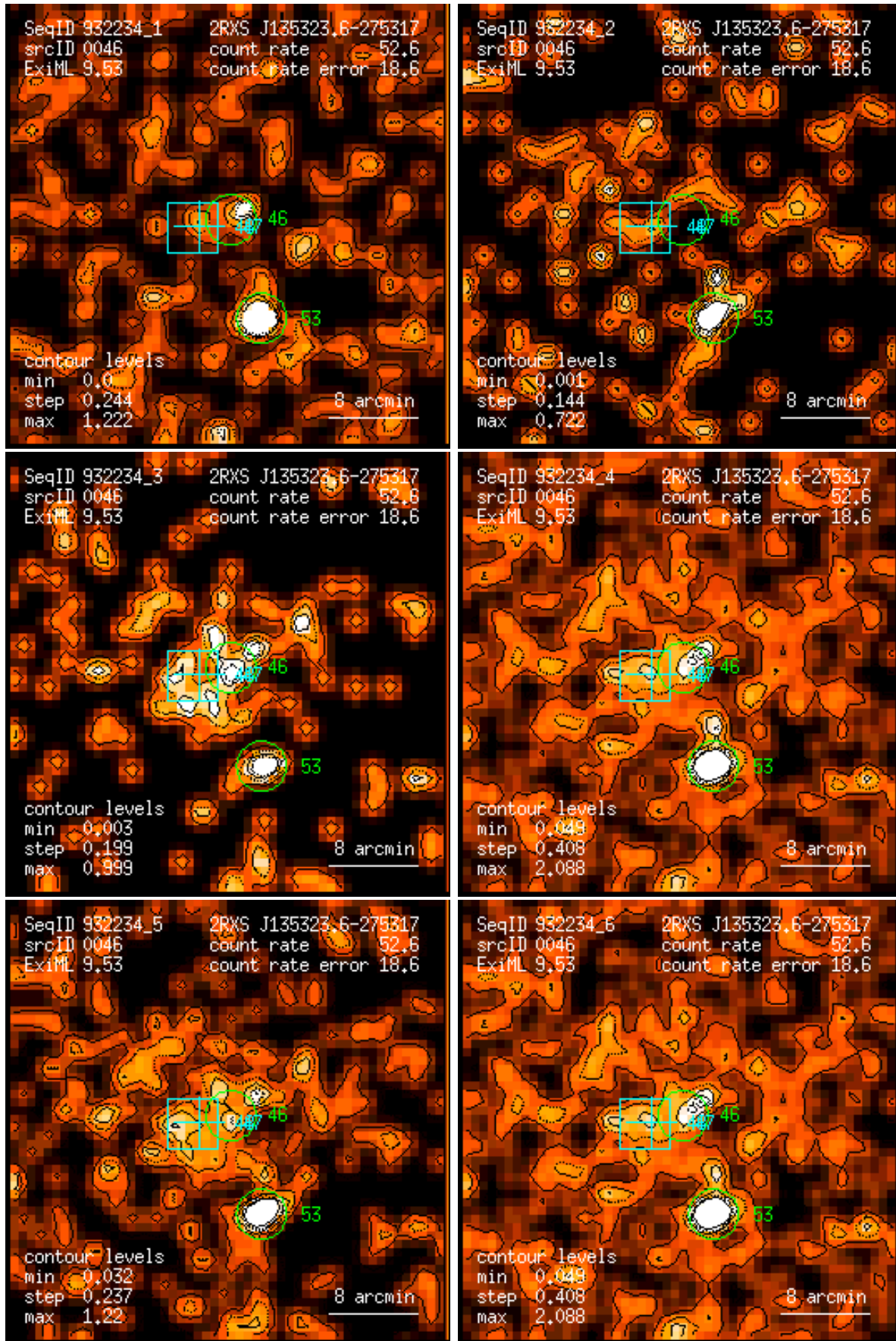
Figure 46: RASS 932234: detection 0046: band rate images, Gaussian filter: (1) PSPC channels 11 – 41, (2) 52 – 90, (3) 91 – 201, (4) 11 – 235, (5) 52 – 201, (6) 11 – 201. Broad band rates in counts/ks. Band rate contour levels in counts/ks/arcmin 2 .
