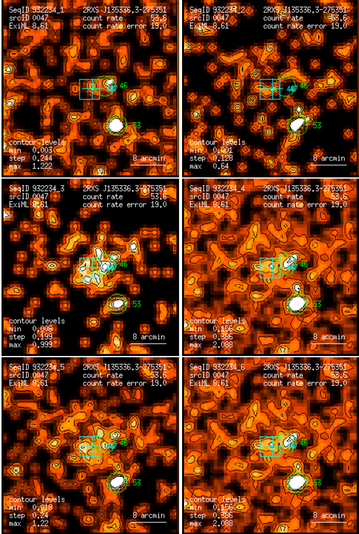
Figure 47: RASS 932234: detection 0047: band rate images, Gaussian filter: (1) PSPC channels 11 – 41, (2) 52 – 90, (3) 91 – 201, (4) 11 – 235, (5) 52 – 201, (6) 11 – 201. Broad band rates in counts/ks. Band rate contour levels in counts/ks/arcmin 2 .
