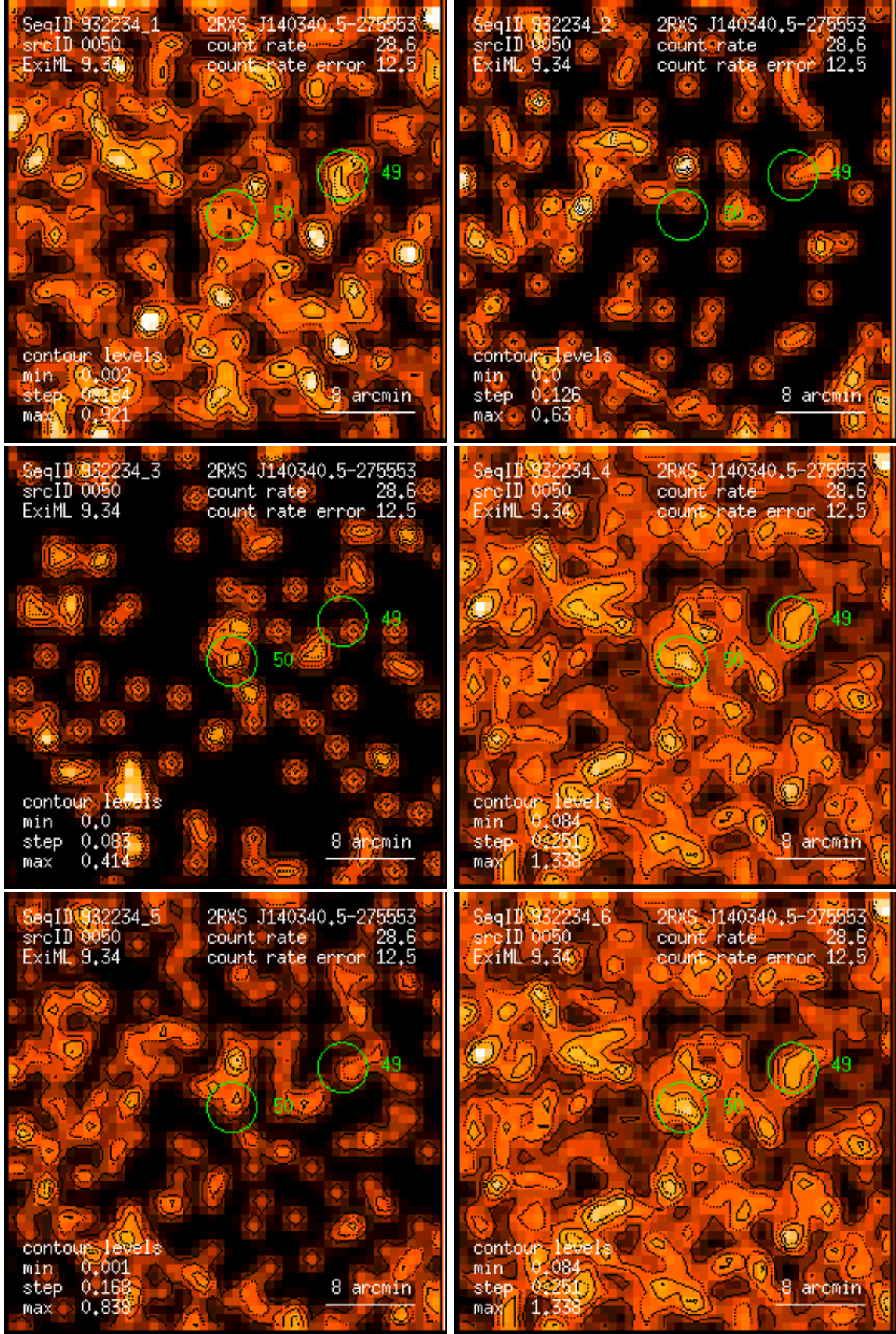
Figure 50: RASS 932234: detection 0050: band rate images, Gaussian filter: (1) PSPC channels 11 – 41, (2) 52 – 90, (3) 91 – 201, (4) 11 – 235, (5) 52 – 201, (6) 11 – 201. Broad band rates in counts/ks. Band rate contour levels in counts/ks/arcmin 2 .
