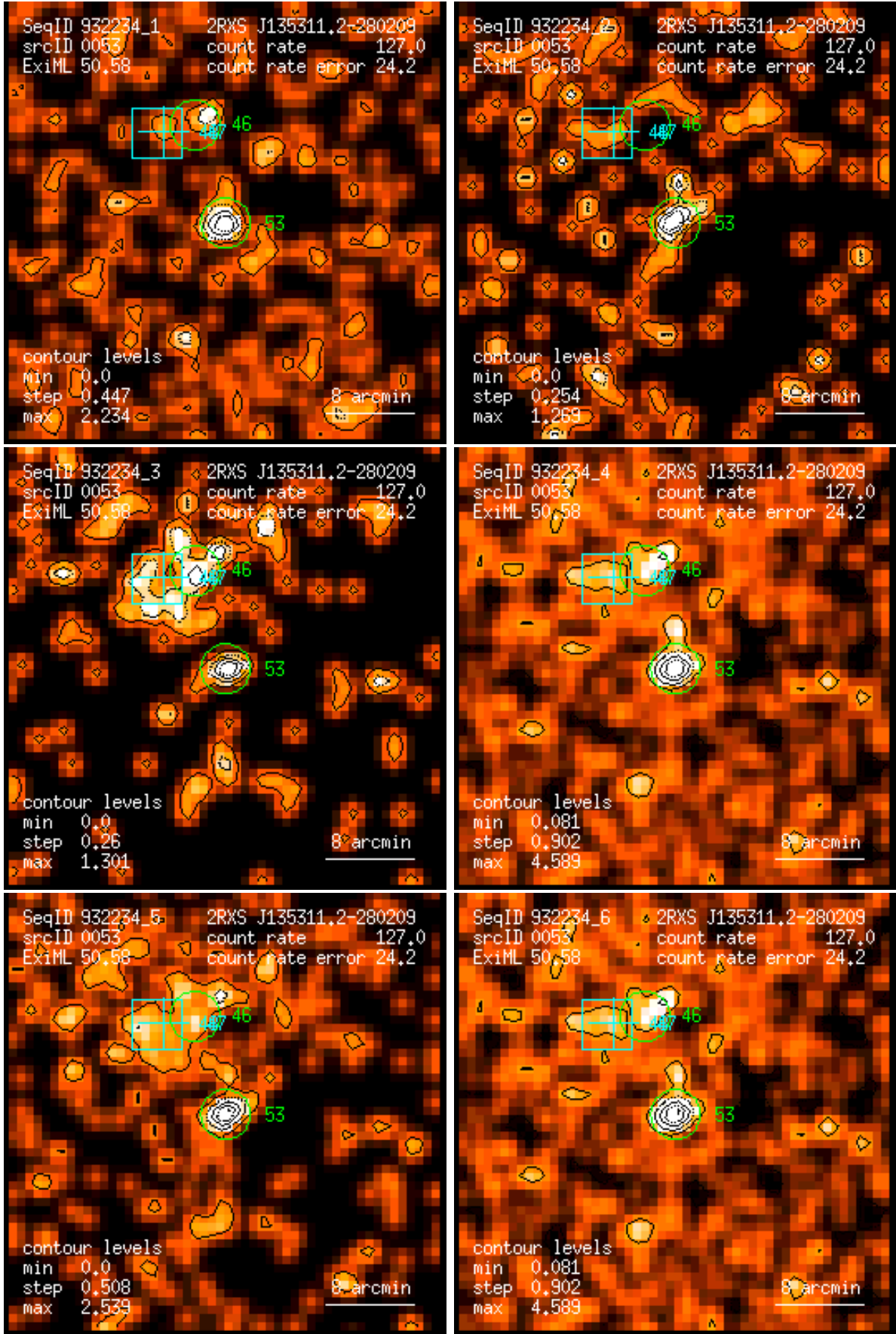
Figure 53: RASS 932234: detection 0053: band rate images, Gaussian filter: (1) PSPC channels 11 – 41, (2) 52 – 90, (3) 91 – 201, (4) 11 – 235, (5) 52 – 201, (6) 11 – 201. Broad band rates in counts/ks. Band rate contour levels in counts/ks/arcmin 2 .
