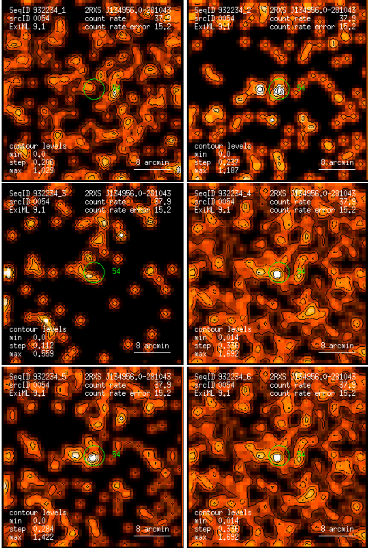
Figure 54: RASS 932234: detection 0054: band rate images, Gaussian filter: (1) PSPC channels 11 – 41, (2) 52 – 90, (3) 91 – 201, (4) 11 – 235, (5) 52 – 201, (6) 11 – 201. Broad band rates in counts/ks. Band rate contour levels in counts/ks/arcmin 2 .
