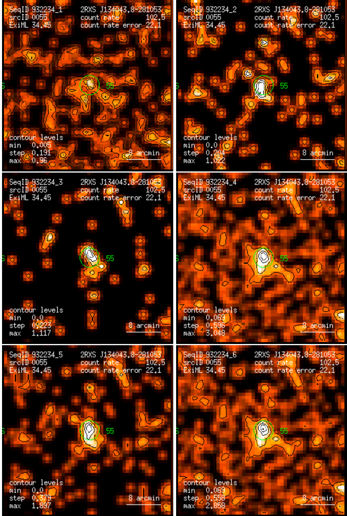
Figure 55: RASS 932234: detection 0055: band rate images, Gaussian filter: (1) PSPC channels 11 – 41, (2) 52 – 90, (3) 91 – 201, (4) 11 – 235, (5) 52 – 201, (6) 11 – 201. Broad band rates in counts/ks. Band rate contour levels in counts/ks/arcmin 2 .
