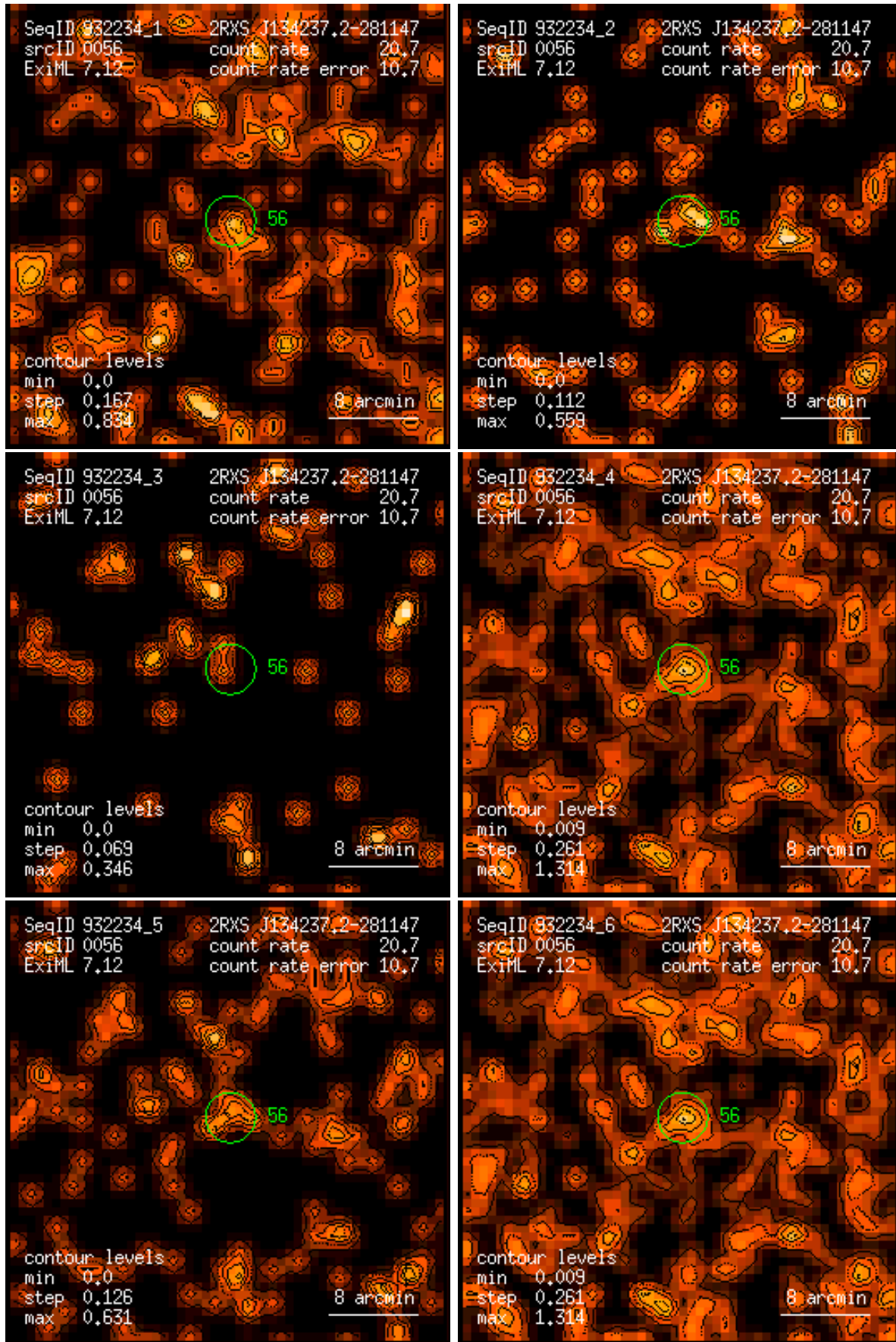
Figure 56: RASS 932234: detection 0056: band rate images, Gaussian filter: (1) PSPC channels 11 – 41, (2) 52 – 90, (3) 91 – 201, (4) 11 – 235, (5) 52 – 201, (6) 11 – 201. Broad band rates in counts/ks. Band rate contour levels in counts/ks/arcmin 2 .
