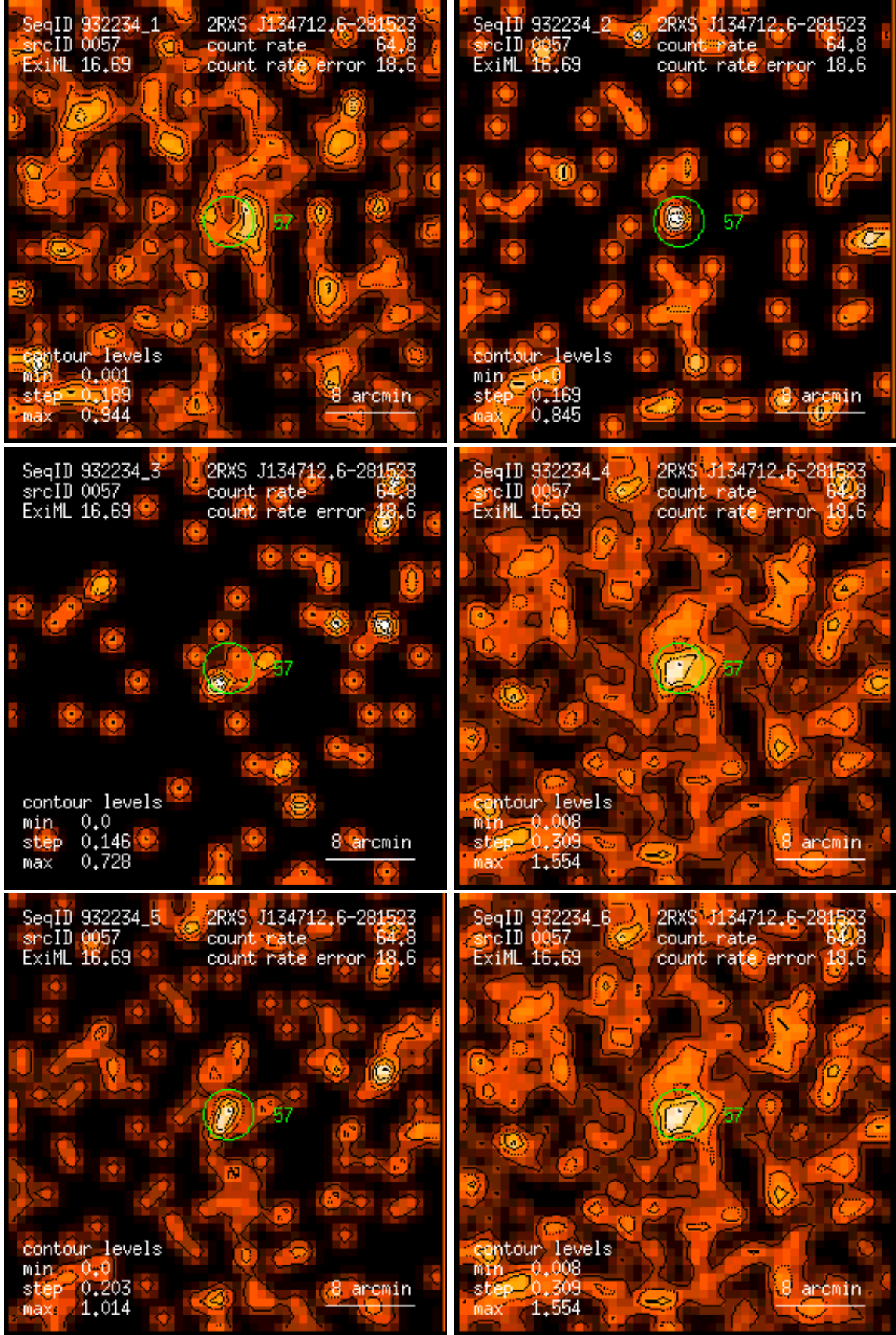
Figure 57: RASS 932234: detection 0057: band rate images, Gaussian filter: (1) PSPC channels 11 – 41, (2) 52 – 90, (3) 91 – 201, (4) 11 – 235, (5) 52 – 201, (6) 11 – 201. Broad band rates in counts/ks. Band rate contour levels in counts/ks/arcmin 2 .
