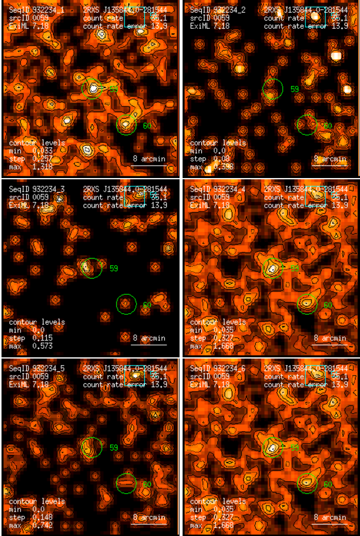
Figure 59: RASS 932234: detection 0059: band rate images, Gaussian filter: (1) PSPC channels 11 – 41, (2) 52 – 90, (3) 91 – 201, (4) 11 – 235, (5) 52 – 201, (6) 11 – 201. Broad band rates in counts/ks. Band rate contour levels in counts/ks/arcmin 2 .
