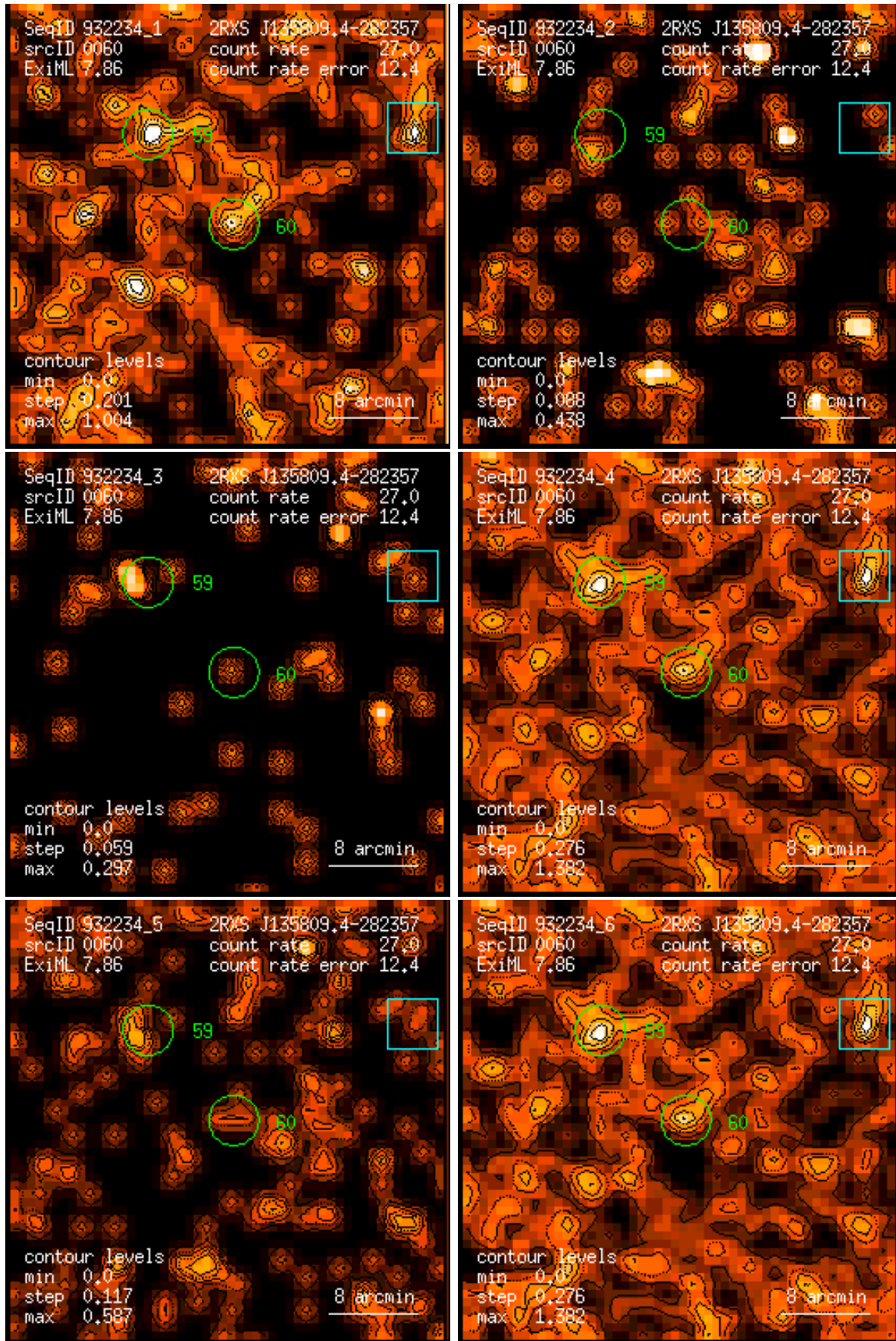
Figure 60: RASS 932234: detection 0060: band rate images, Gaussian filter: (1) PSPC channels 11 – 41, (2) 52 – 90, (3) 91 – 201, (4) 11 – 235, (5) 52 – 201, (6) 11 – 201. Broad band rates in counts/ks. Band rate contour levels in counts/ks/arcmin 2 .
