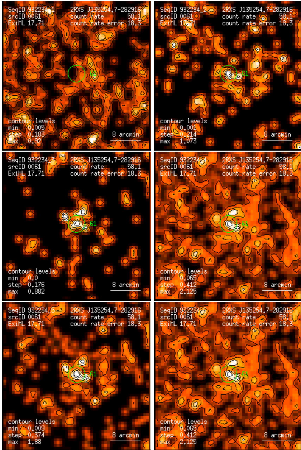
Figure 61: RASS 932234: detection 0061: band rate images, Gaussian filter: (1) PSPC channels 11 – 41, (2) 52 – 90, (3) 91 – 201, (4) 11 – 235, (5) 52 – 201, (6) 11 – 201. Broad band rates in counts/ks. Band rate contour levels in counts/ks/arcmin 2 .
