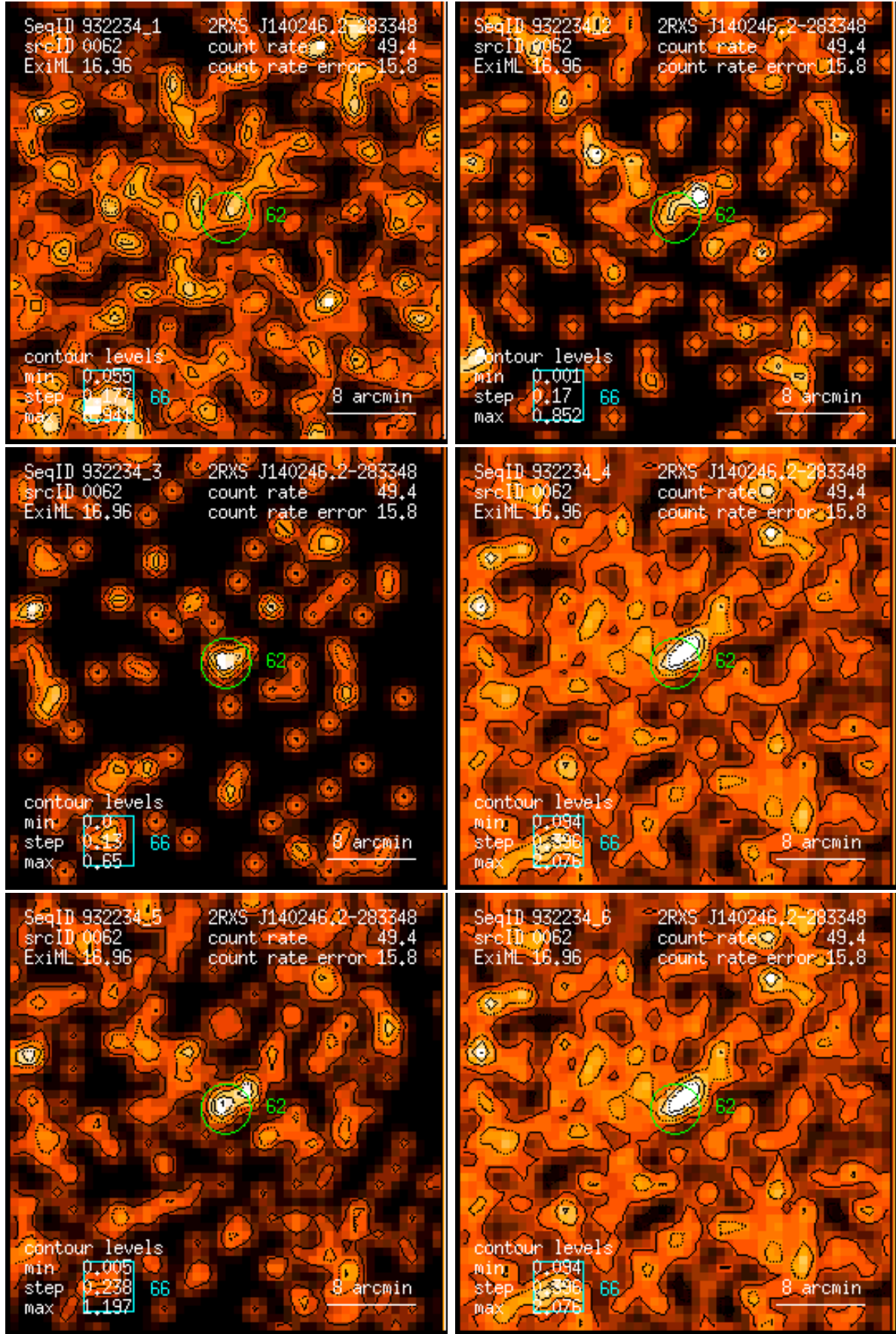
Figure 62: RASS 932234: detection 0062: band rate images, Gaussian filter: (1) PSPC channels 11 – 41, (2) 52 – 90, (3) 91 – 201, (4) 11 – 235, (5) 52 – 201, (6) 11 – 201. Broad band rates in counts/ks. Band rate contour levels in counts/ks/arcmin 2 .
