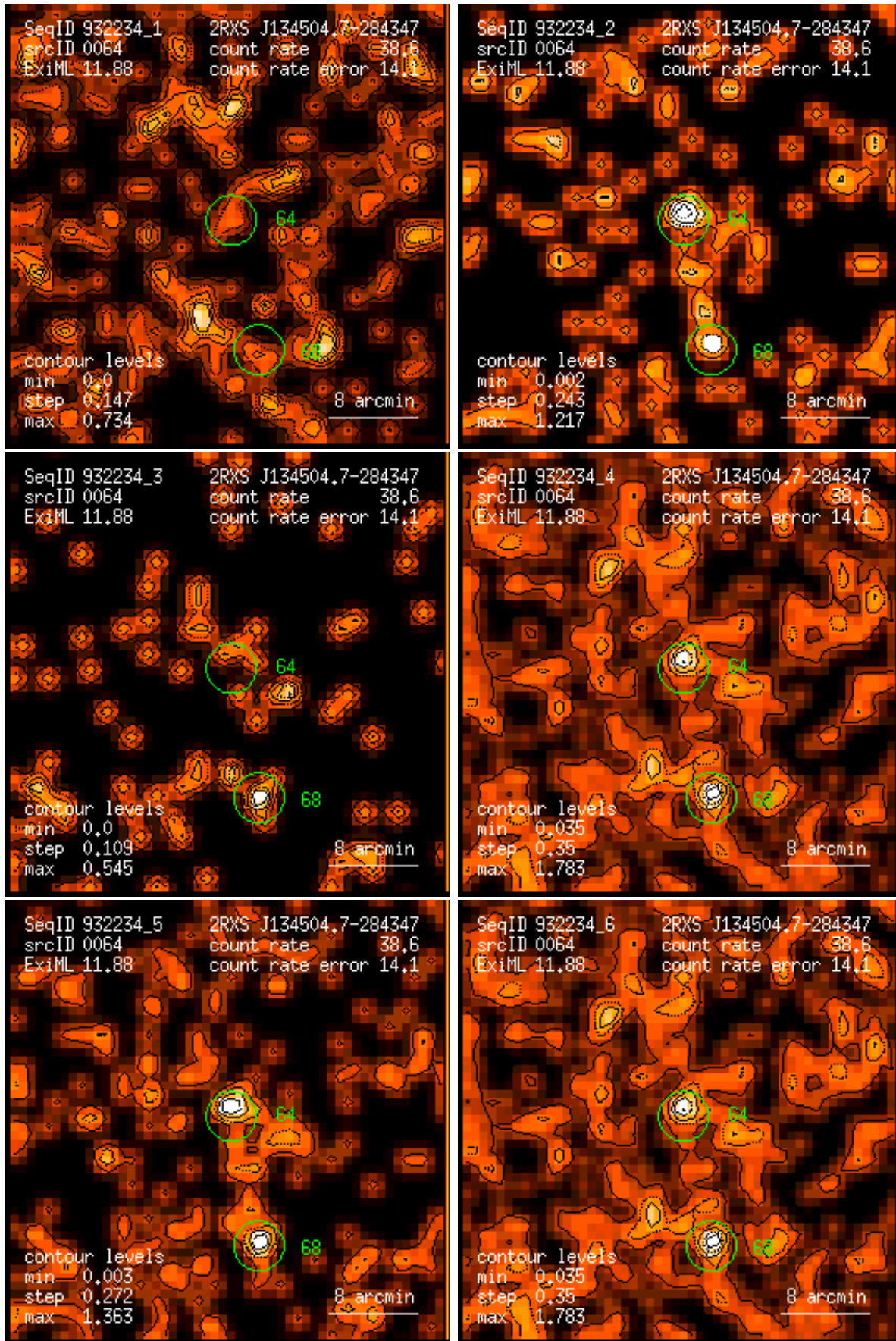
Figure 64: RASS 932234: detection 0064: band rate images, Gaussian filter: (1) PSPC channels 11 – 41, (2) 52 – 90, (3) 91 – 201, (4) 11 – 235, (5) 52 – 201, (6) 11 – 201. Broad band rates in counts/ks. Band rate contour levels in counts/ks/arcmin 2 .
