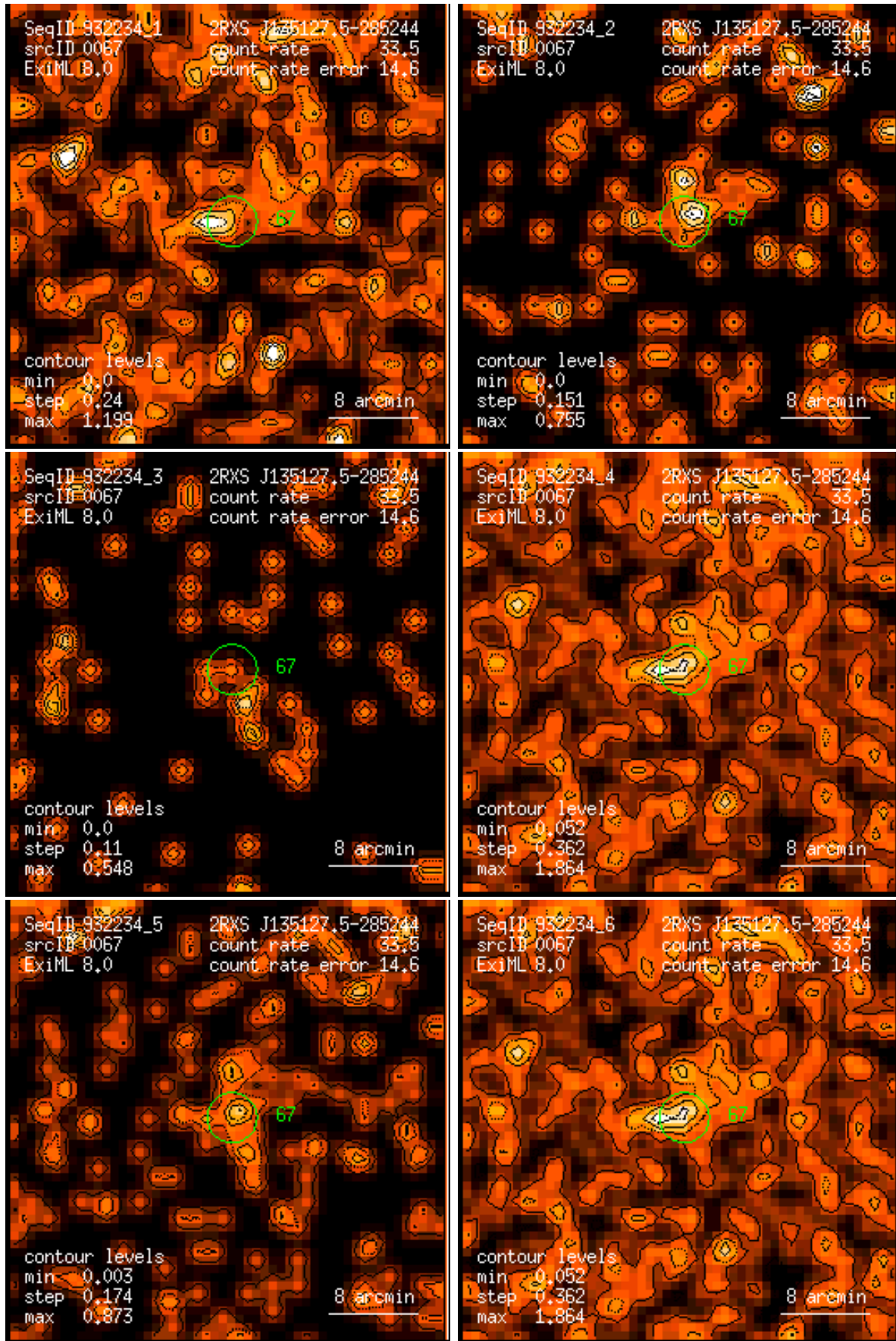
Figure 67: RASS 932234: detection 0067: band rate images, Gaussian filter: (1) PSPC channels 11 – 41, (2) 52 – 90, (3) 91 – 201, (4) 11 – 235, (5) 52 – 201, (6) 11 – 201. Broad band rates in counts/ks. Band rate contour levels in counts/ks/arcmin 2 .
