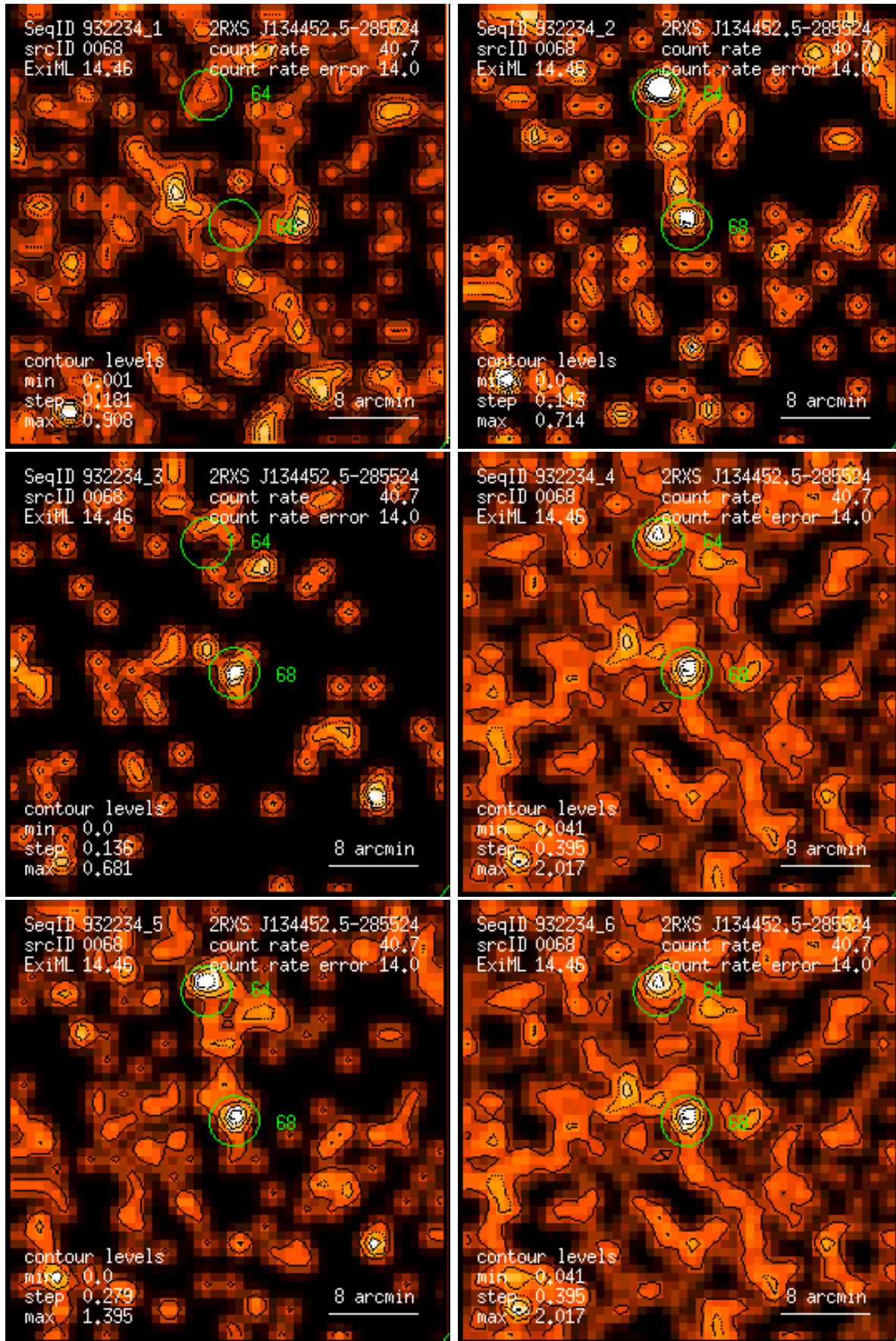
Figure 68: RASS 932234: detection 0068: band rate images, Gaussian filter: (1) PSPC channels 11 – 41, (2) 52 – 90, (3) 91 – 201, (4) 11 – 235, (5) 52 – 201, (6) 11 – 201. Broad band rates in counts/ks. Band rate contour levels in counts/ks/arcmin 2 .
