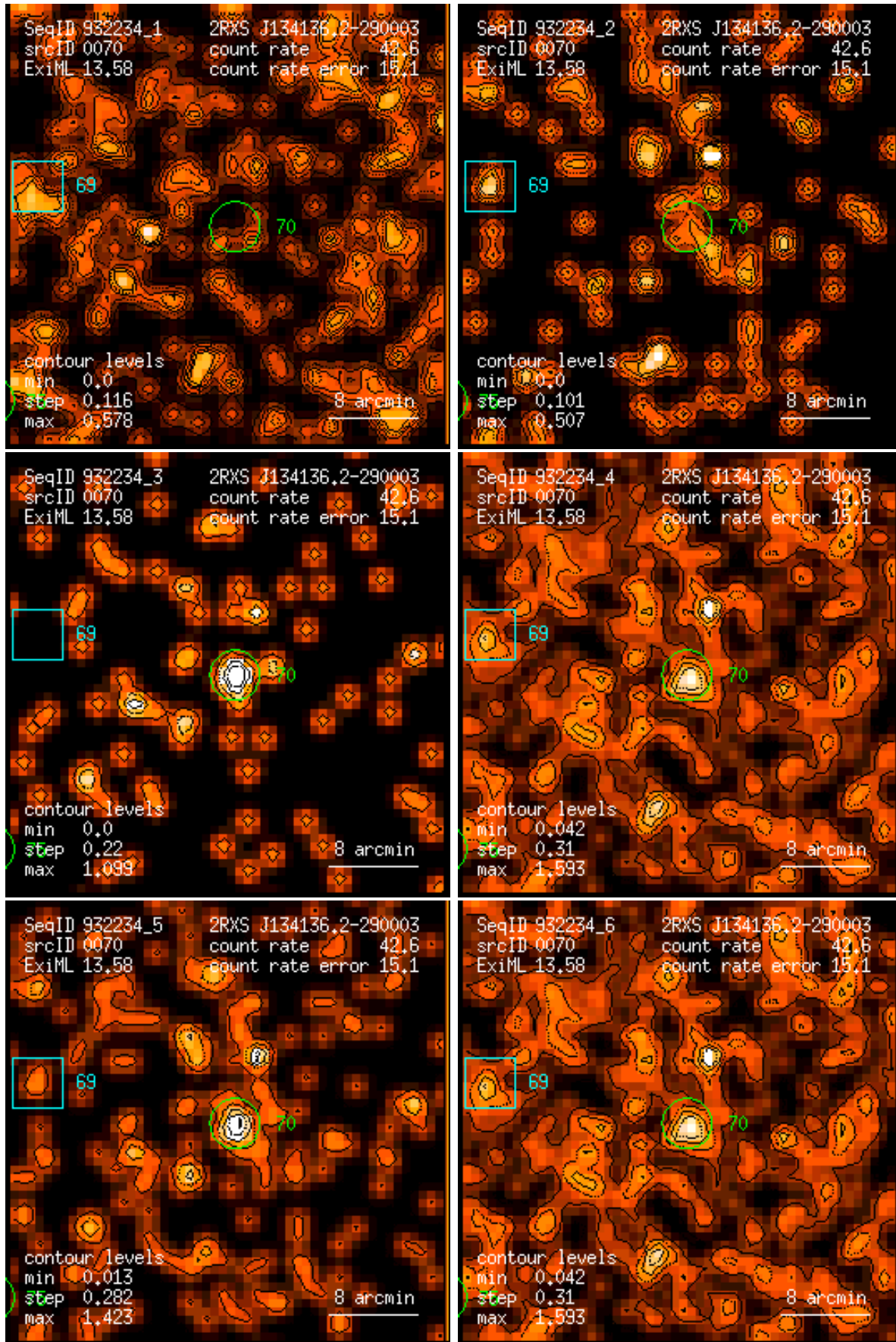
Figure 70: RASS 932234: detection 0070: band rate images, Gaussian filter: (1) PSPC channels 11 – 41, (2) 52 – 90, (3) 91 – 201, (4) 11 – 235, (5) 52 – 201, (6) 11 – 201. Broad band rates in counts/ks. Band rate contour levels in counts/ks/arcmin 2 .
