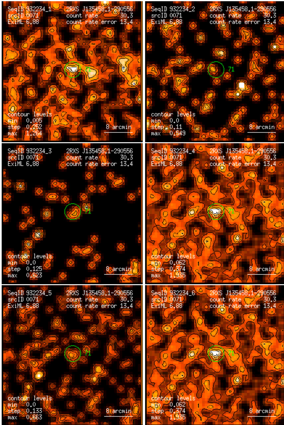
Figure 71: RASS 932234: detection 0071: band rate images, Gaussian filter: (1) PSPC channels 11 – 41, (2) 52 – 90, (3) 91 – 201, (4) 11 – 235, (5) 52 – 201, (6) 11 – 201. Broad band rates in counts/ks. Band rate contour levels in counts/ks/arcmin 2 .
