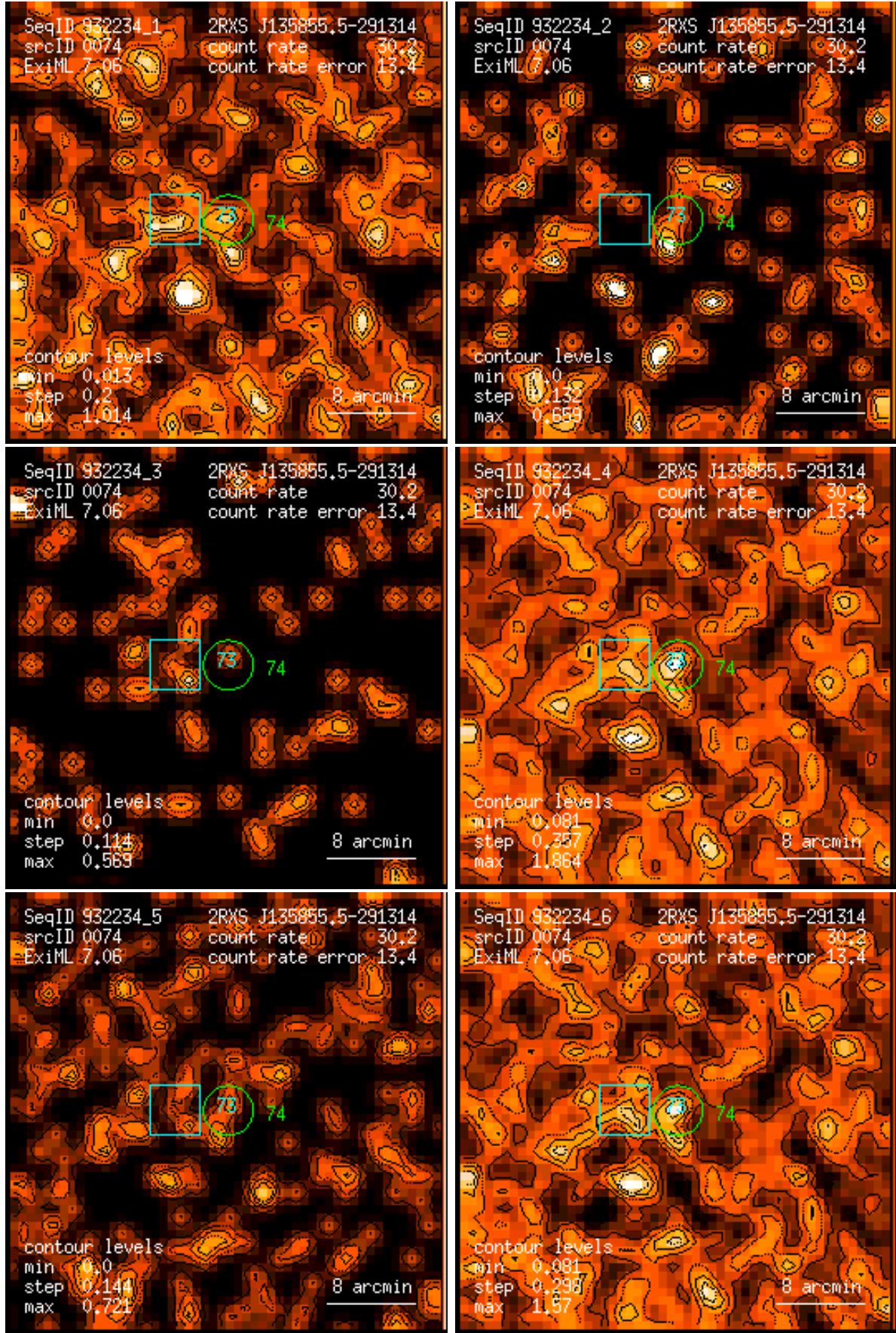
Figure 74: RASS 932234: detection 0074: band rate images, Gaussian filter: (1) PSPC channels 11 – 41, (2) 52 – 90, (3) 91 – 201, (4) 11 – 235, (5) 52 – 201, (6) 11 – 201. Broad band rates in counts/ks. Band rate contour levels in counts/ks/arcmin 2 .
