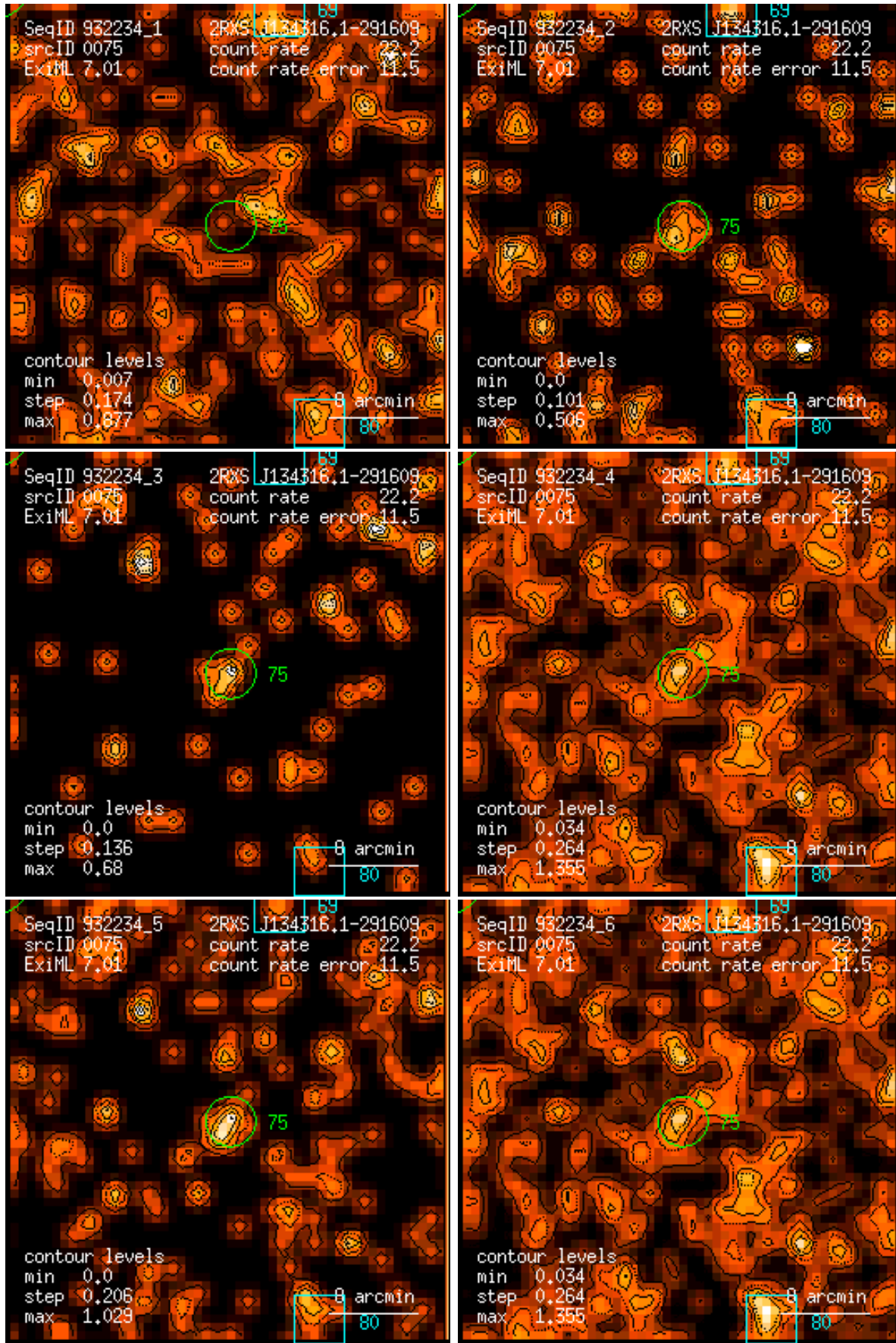
Figure 75: RASS 932234: detection 0075: band rate images, Gaussian filter: (1) PSPC channels 11 – 41, (2) 52 – 90, (3) 91 – 201, (4) 11 – 235, (5) 52 – 201, (6) 11 – 201. Broad band rates in counts/ks. Band rate contour levels in counts/ks/arcmin 2 .
