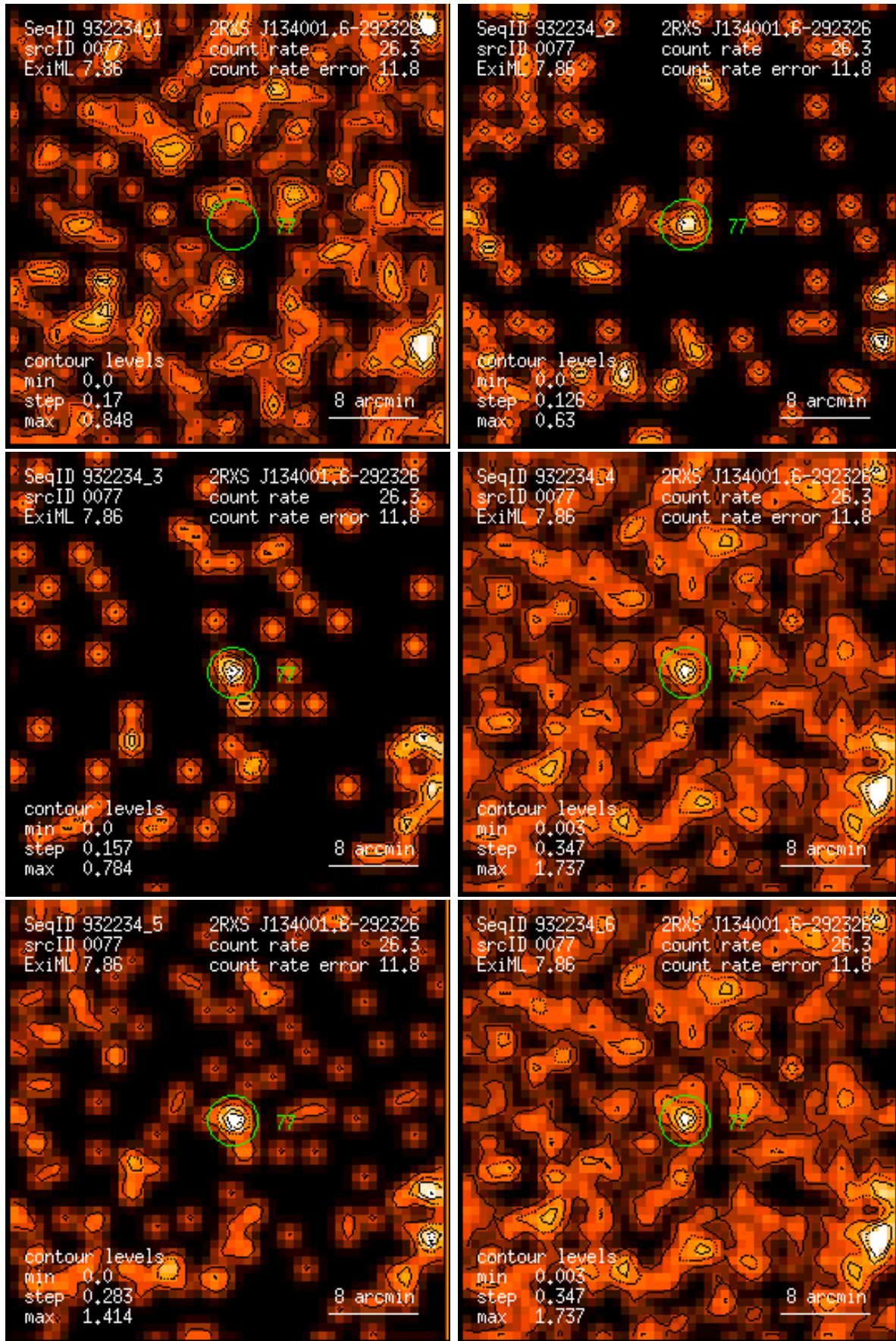
Figure 77: RASS 932234: detection 0077: band rate images, Gaussian filter: (1) PSPC channels 11 – 41, (2) 52 – 90, (3) 91 – 201, (4) 11 – 235, (5) 52 – 201, (6) 11 – 201. Broad band rates in counts/ks. Band rate contour levels in counts/ks/arcmin 2 .
