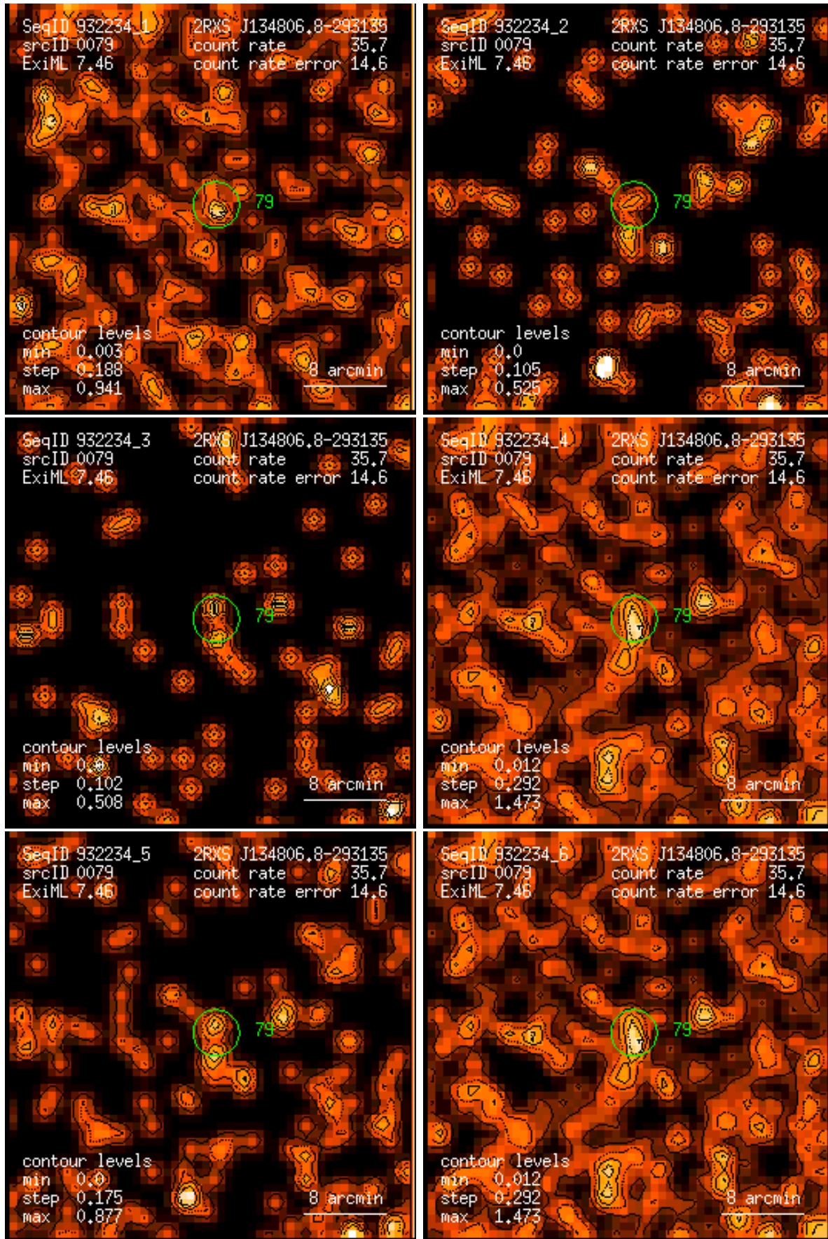
Figure 79: RASS 932234: detection 0079: band rate images, Gaussian filter: (1) PSPC channels 11 – 41, (2) 52 – 90, (3) 91 – 201, (4) 11 – 235, (5) 52 – 201, (6) 11 – 201. Broad band rates in counts/ks. Band rate contour levels in counts/ks/arcmin 2 .
