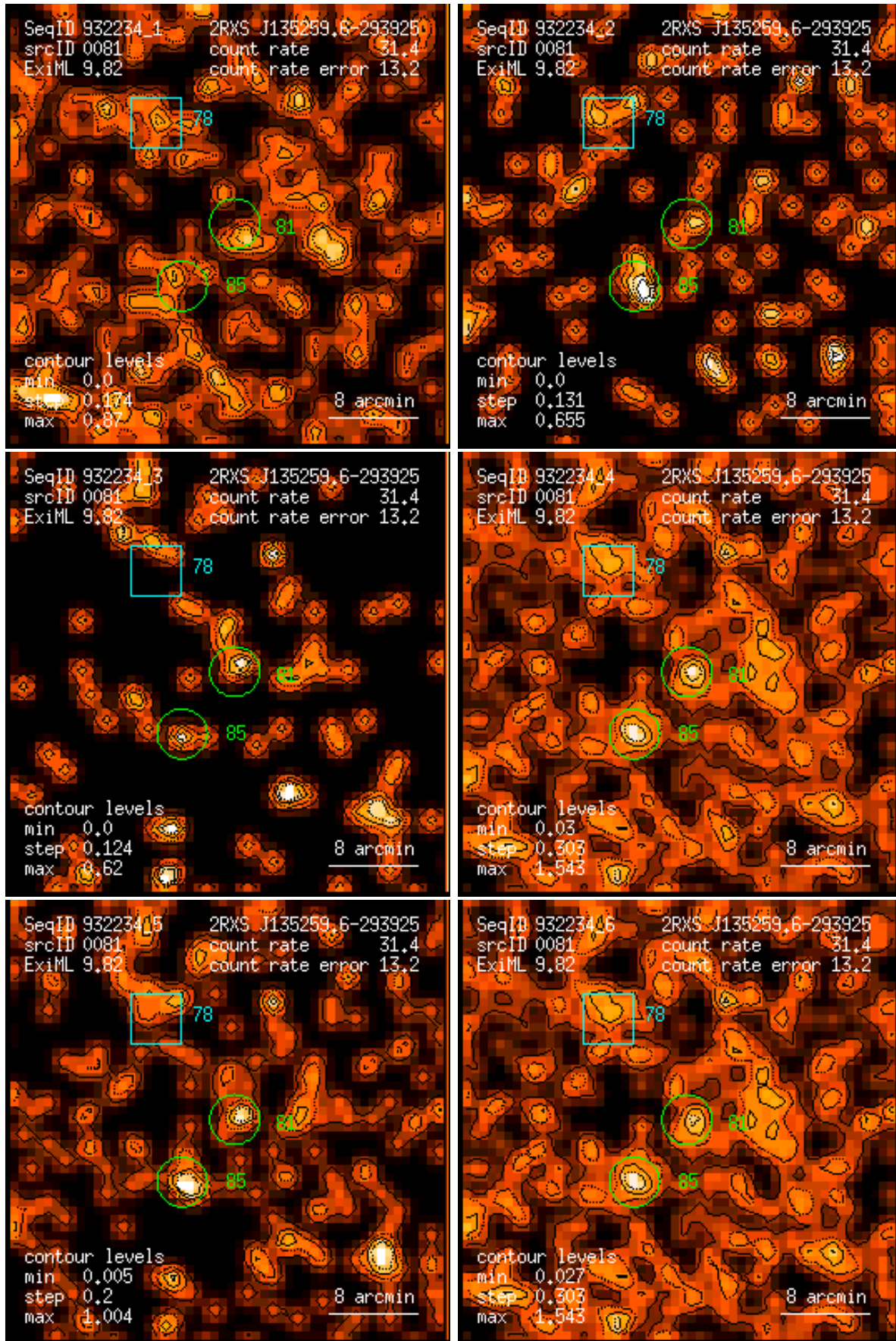
Figure 81: RASS 932234: detection 0081: band rate images, Gaussian filter: (1) PSPC channels 11 – 41, (2) 52 – 90, (3) 91 – 201, (4) 11 – 235, (5) 52 – 201, (6) 11 – 201. Broad band rates in counts/ks. Band rate contour levels in counts/ks/arcmin 2 .
