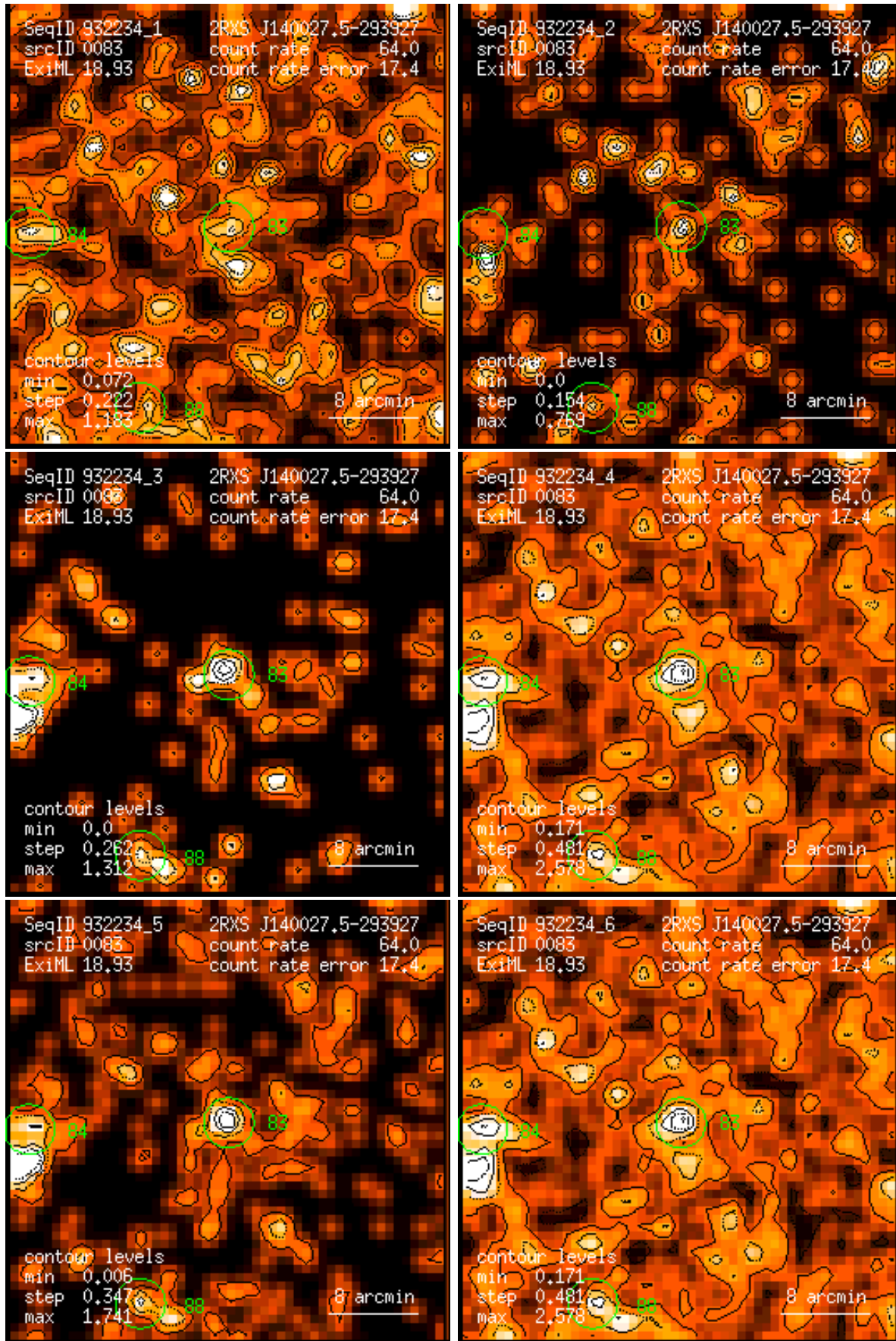
Figure 83: RASS 932234: detection 0083: band rate images, Gaussian filter: (1) PSPC channels 11 – 41, (2) 52 – 90, (3) 91 – 201, (4) 11 – 235, (5) 52 – 201, (6) 11 – 201. Broad band rates in counts/ks. Band rate contour levels in counts/ks/arcmin 2 .
