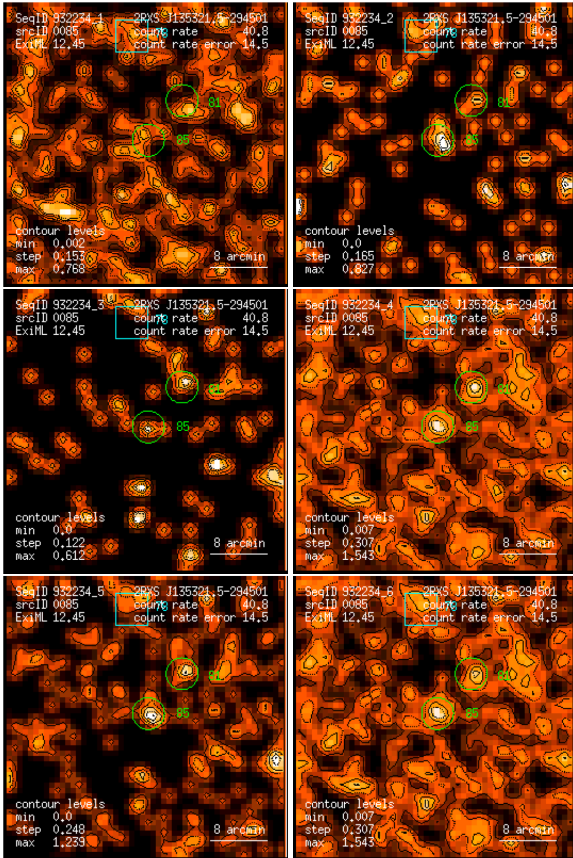
Figure 85: RASS 932234: detection 0085: band rate images, Gaussian filter: (1) PSPC channels 11 – 41, (2) 52 – 90, (3) 91 – 201, (4) 11 – 235, (5) 52 – 201, (6) 11 – 201. Broad band rates in counts/ks. Band rate contour levels in counts/ks/arcmin 2 .
