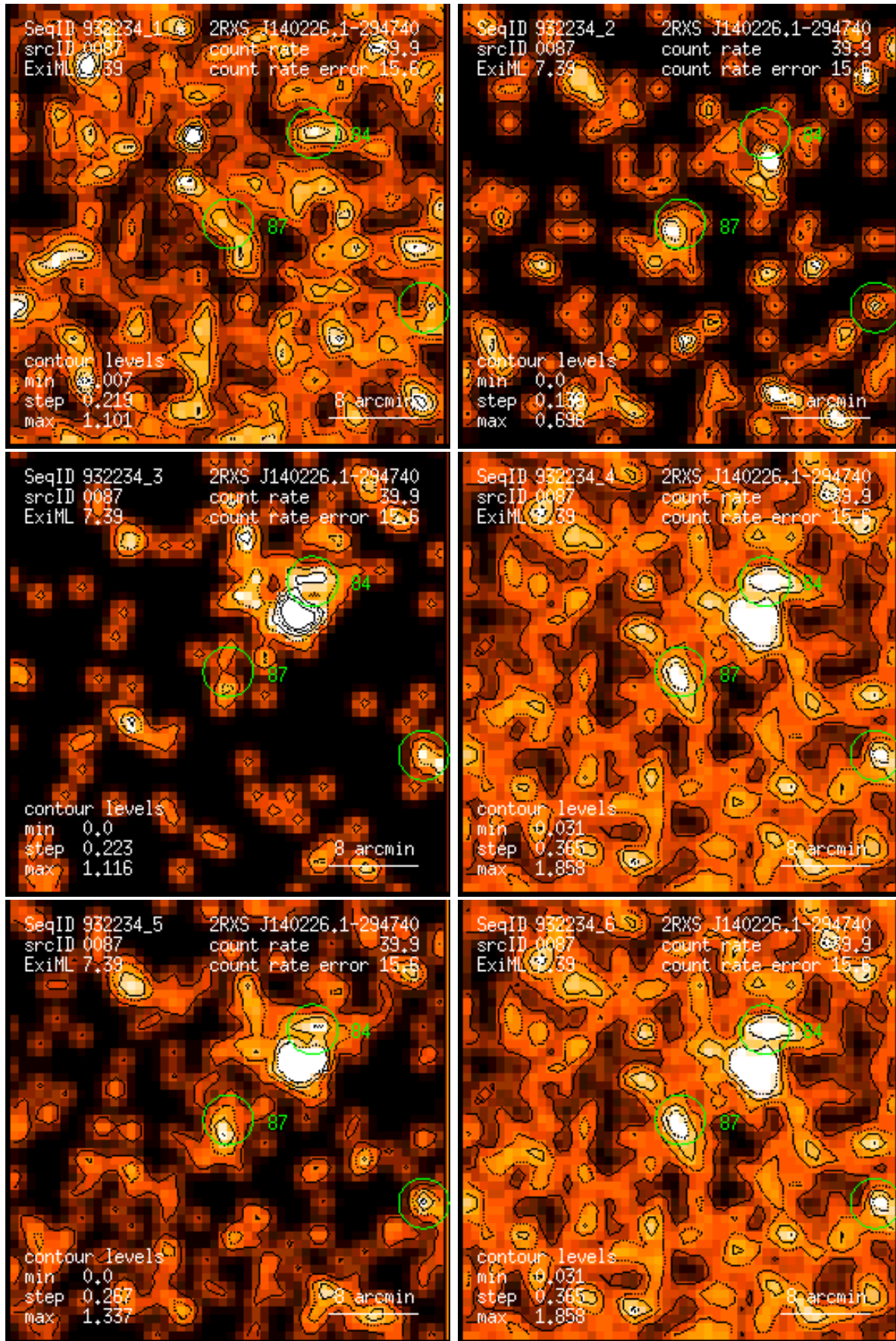
Figure 87: RASS 932234: detection 0087: band rate images, Gaussian filter: (1) PSPC channels 11 – 41, (2) 52 – 90, (3) 91 – 201, (4) 11 – 235, (5) 52 – 201, (6) 11 – 201. Broad band rates in counts/ks. Band rate contour levels in counts/ks/arcmin 2 .
