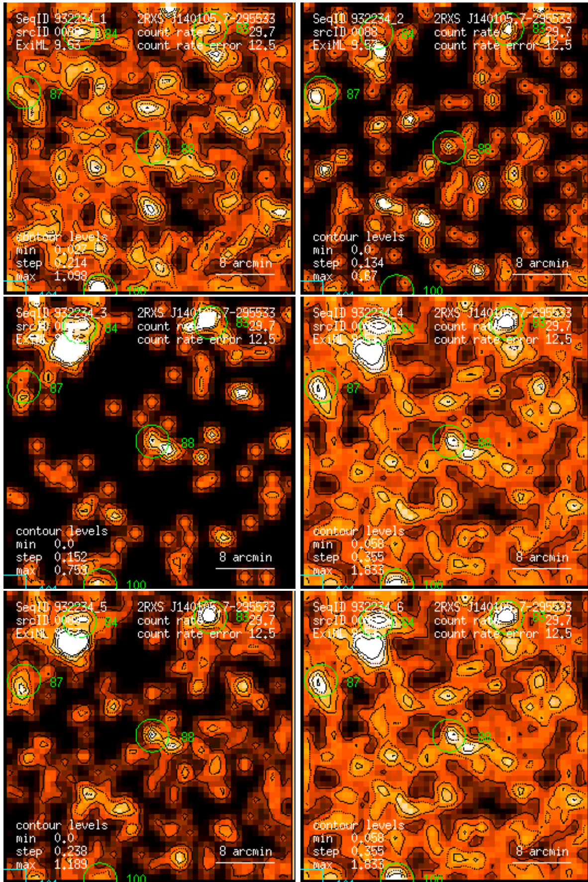
Figure 88: RASS 932234: detection 0088: band rate images, Gaussian filter: (1) PSPC channels 11 – 41, (2) 52 – 90, (3) 91 – 201, (4) 11 – 235, (5) 52 – 201, (6) 11 – 201. Broad band rates in counts/ks. Band rate contour levels in counts/ks/arcmin 2 .
