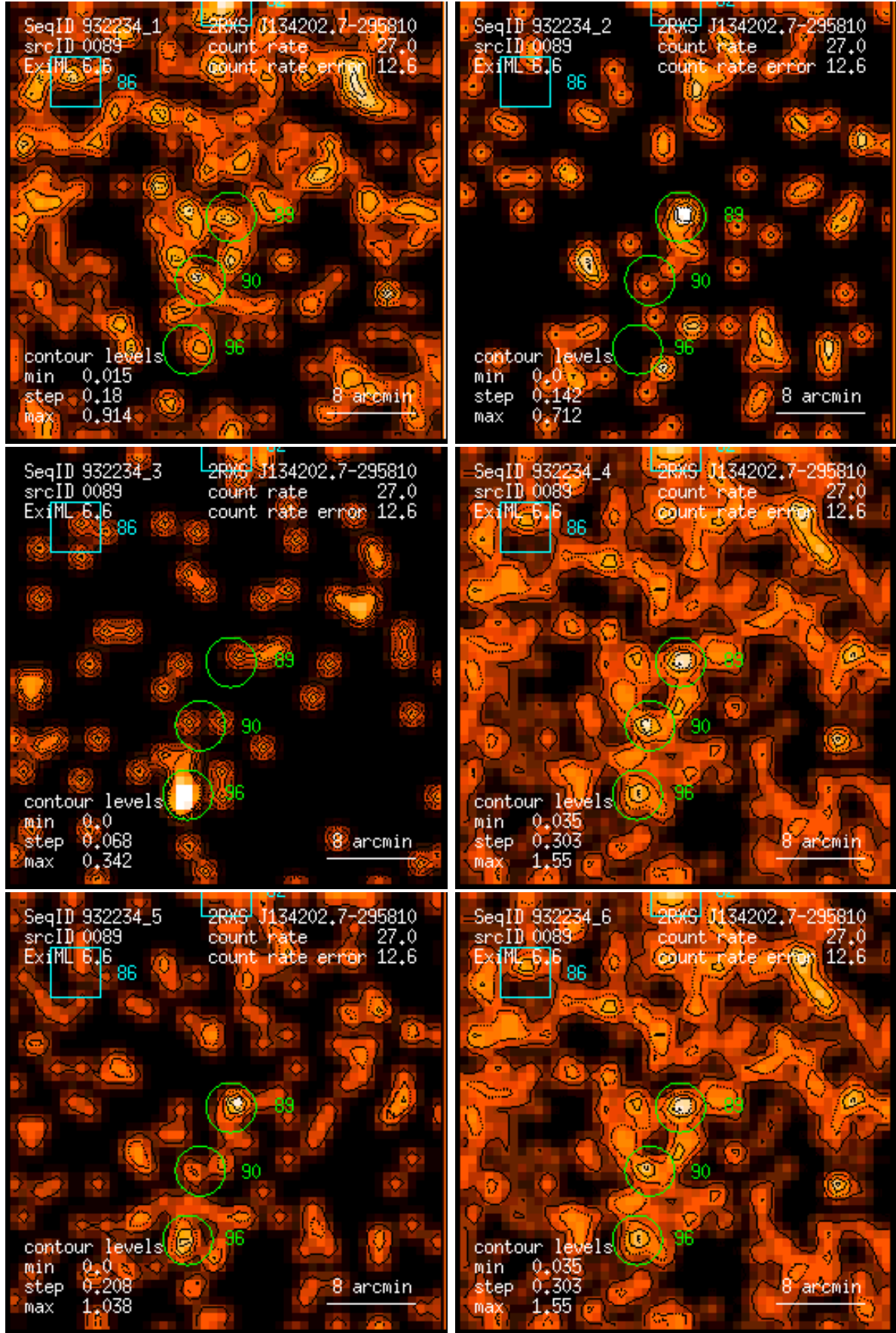
Figure 89: RASS 932234: detection 0089: band rate images, Gaussian filter: (1) PSPC channels 11 – 41, (2) 52 – 90, (3) 91 – 201, (4) 11 – 235, (5) 52 – 201, (6) 11 – 201. Broad band rates in counts/ks. Band rate contour levels in counts/ks/arcmin 2 .
