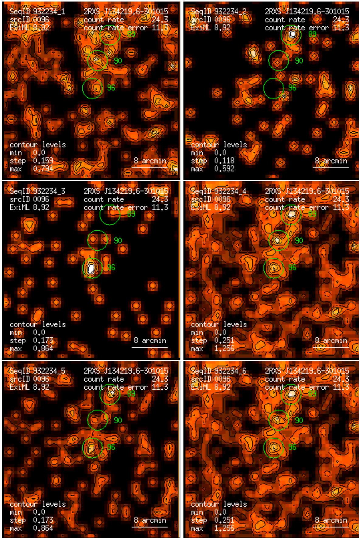
Figure 96: RASS 932234: detection 0096: band rate images, Gaussian filter: (1) PSPC channels 11 – 41, (2) 52 – 90, (3) 91 – 201, (4) 11 – 235, (5) 52 – 201, (6) 11 – 201. Broad band rates in counts/ks. Band rate contour levels in counts/ks/arcmin 2 .
