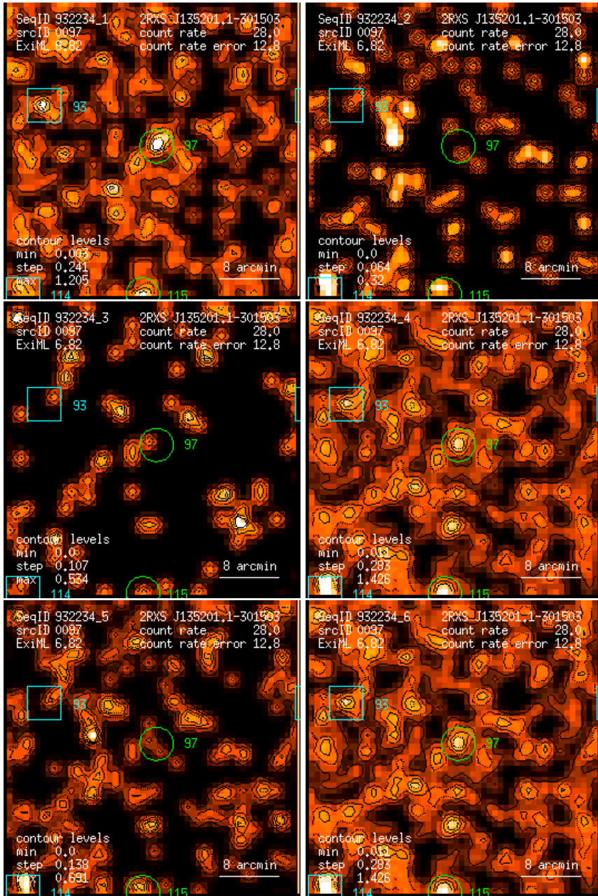
Figure 97: RASS 932234: detection 0097: band rate images, Gaussian filter: (1) PSPC channels 11 – 41, (2) 52 – 90, (3) 91 – 201, (4) 11 – 235, (5) 52 – 201, (6) 11 – 201. Broad band rates in counts/ks. Band rate contour levels in counts/ks/arcmin 2 .
