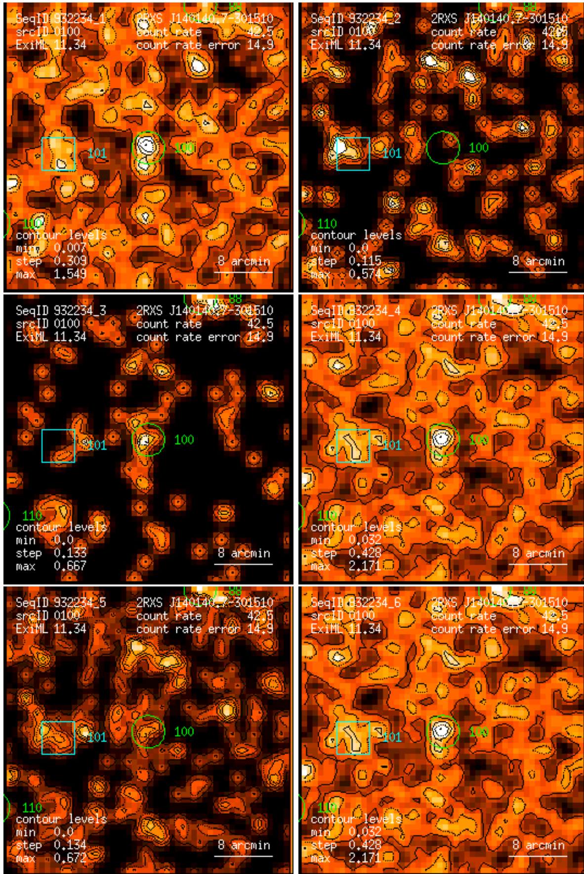
Figure 100: RASS 932234: detection 0100: band rate images, Gaussian filter: (1) PSPC channels 11 – 41, (2) 52 – 90, (3) 91 – 201, (4) 11 – 235, (5) 52 – 201, (6) 11 – 201. Broad band rates in counts/ks. Band rate contour levels in counts/ks/arcmin 2 .
