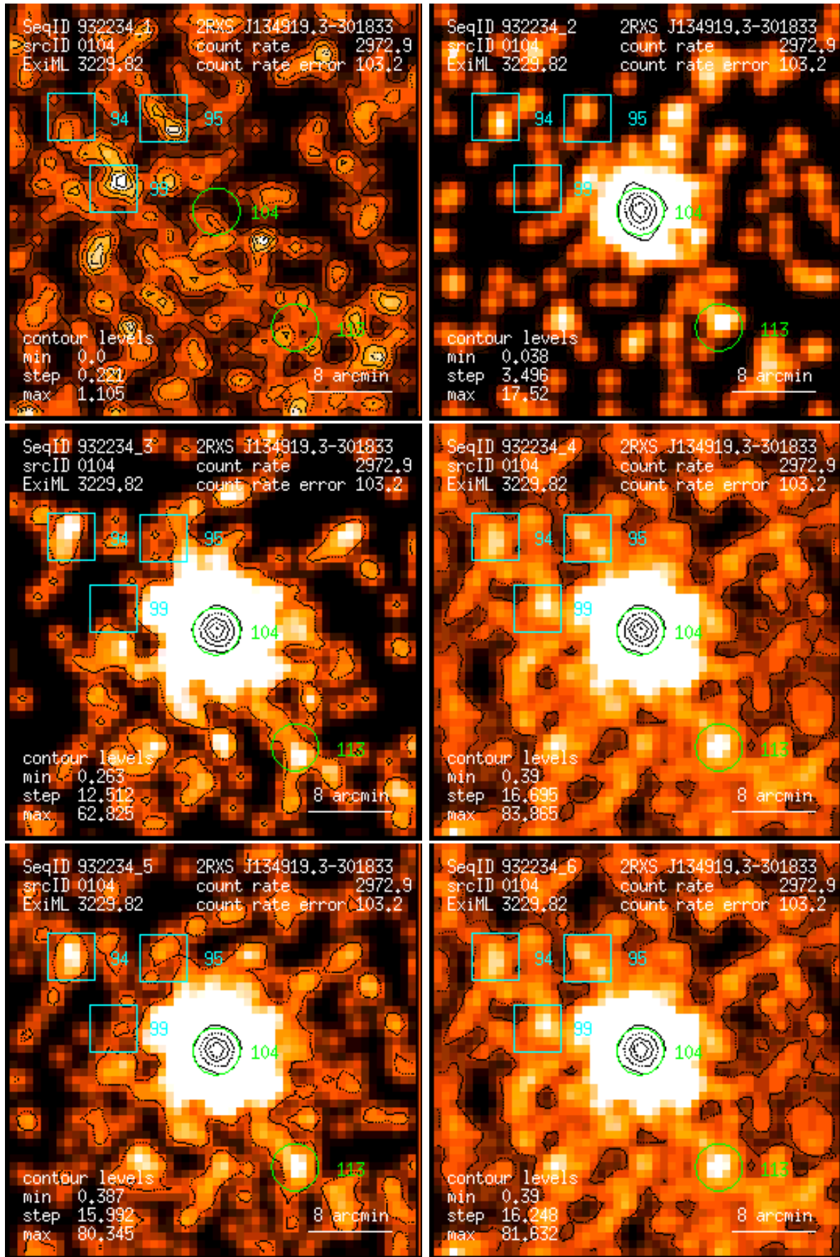
Figure 104: RASS 932234: detection 0104: band rate images, Gaussian filter: (1) PSPC channels 11 – 41, (2) 52 – 90, (3) 91 – 201, (4) 11 – 235, (5) 52 – 201, (6) 11 – 201. Broad band rates in counts/ks. Band rate contour levels in counts/ks/arcmin 2 .
