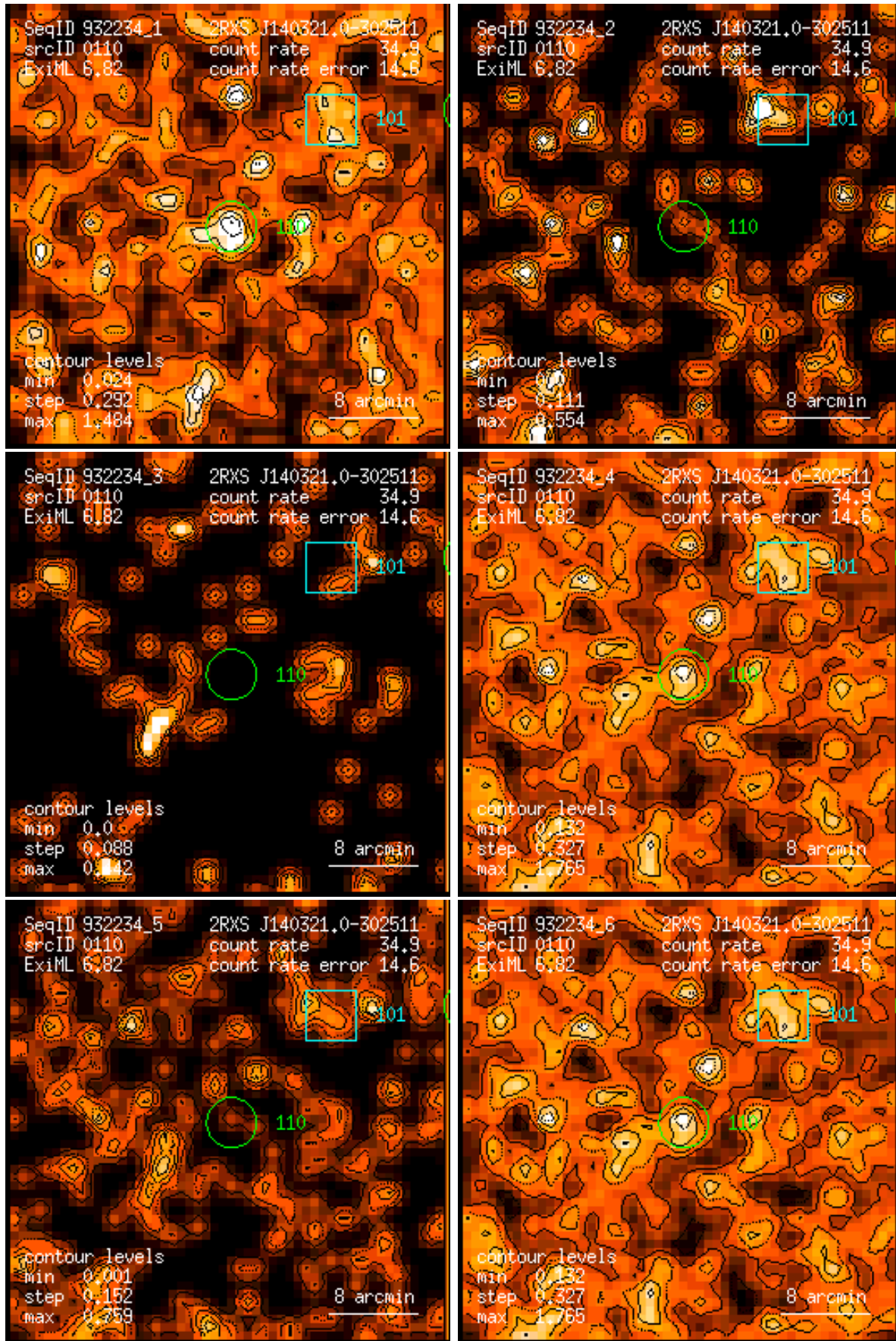
Figure 110: RASS 932234: detection 0110: band rate images, Gaussian filter: (1) PSPC channels 11 – 41, (2) 52 – 90, (3) 91 – 201, (4) 11 – 235, (5) 52 – 201, (6) 11 – 201. Broad band rates in counts/ks. Band rate contour levels in counts/ks/arcmin 2 .
