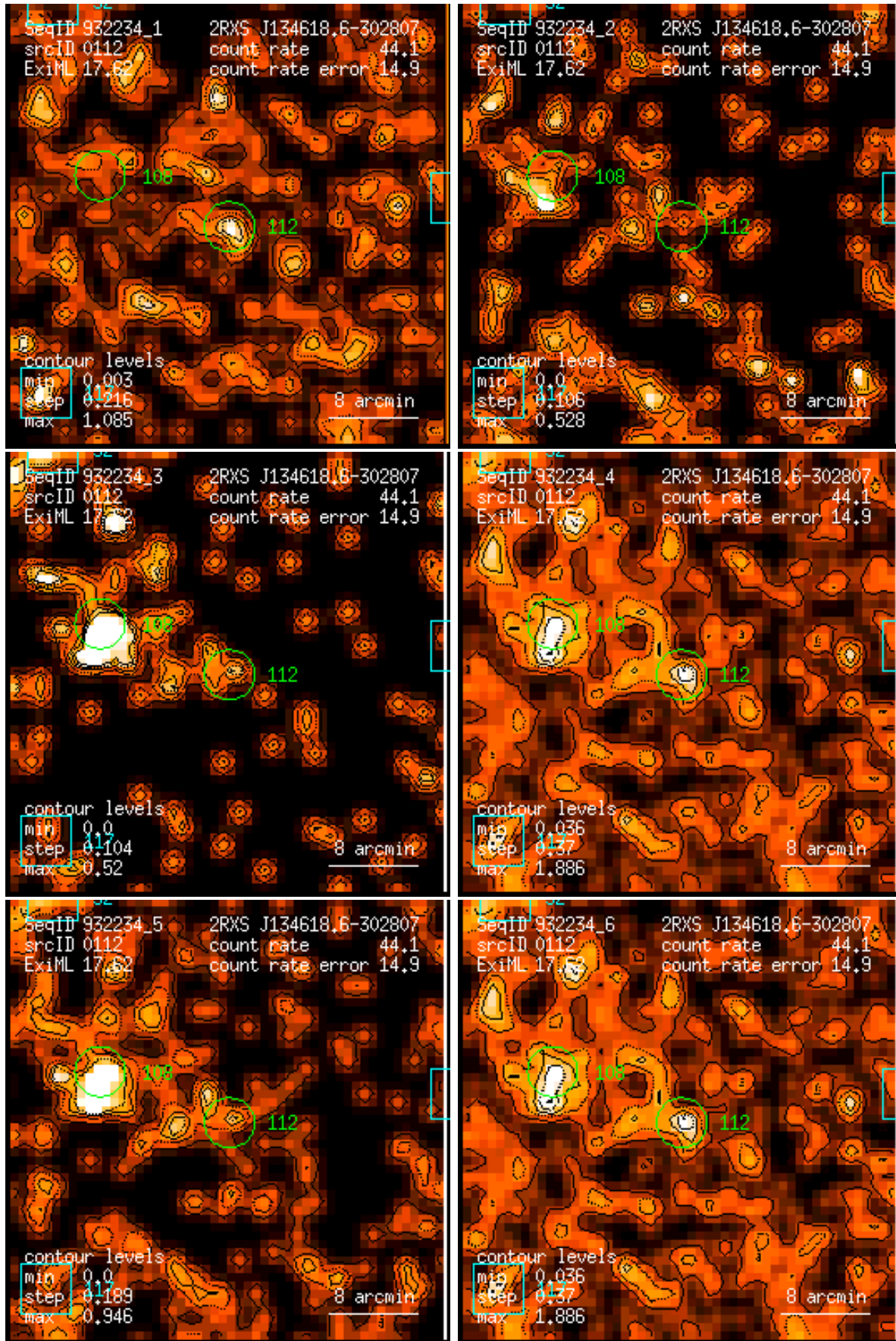
Figure 112: RASS 932234: detection 0112: band rate images, Gaussian filter: (1) PSPC channels 11 – 41, (2) 52 – 90, (3) 91 – 201, (4) 11 – 235, (5) 52 – 201, (6) 11 – 201. Broad band rates in counts/ks. Band rate contour levels in counts/ks/arcmin 2 .
