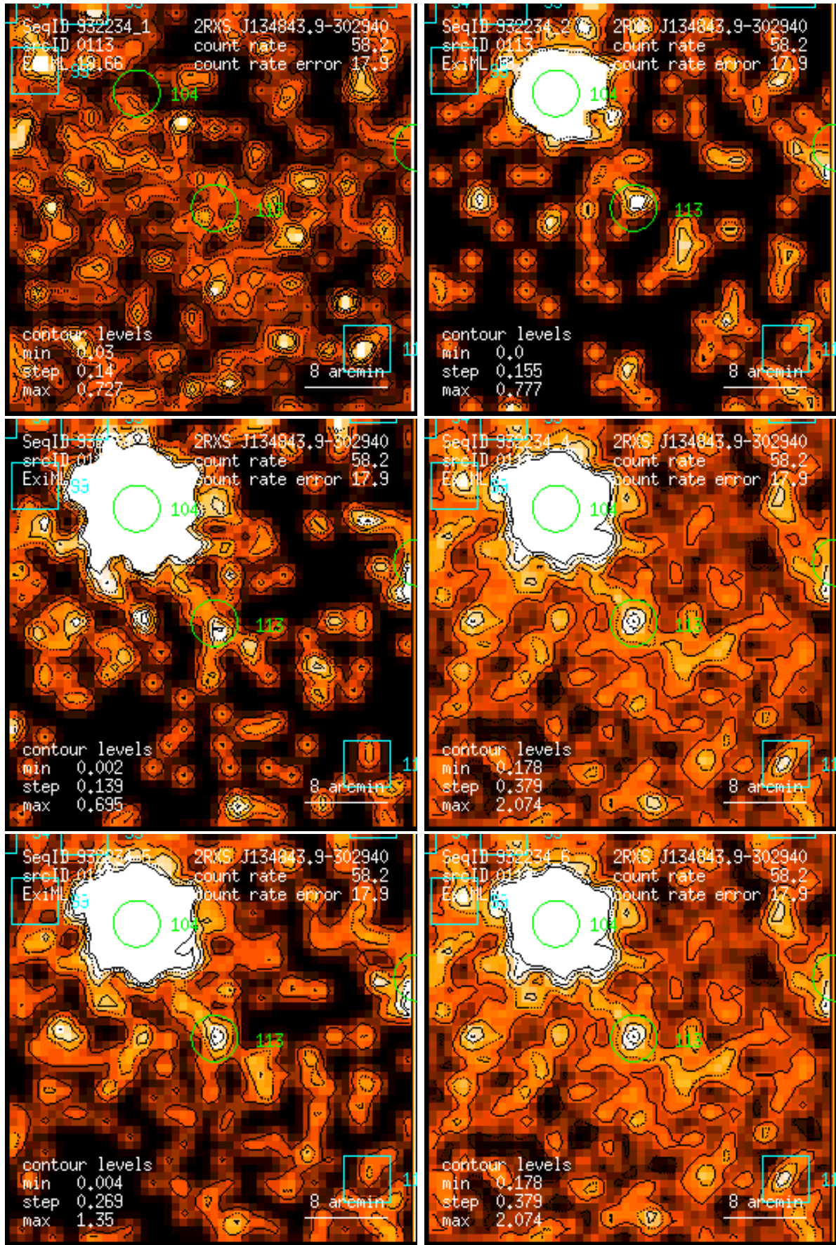
Figure 113: RASS 932234: detection 0113: band rate images, Gaussian filter: (1) PSPC channels 11 – 41, (2) 52 – 90, (3) 91 – 201, (4) 11 – 235, (5) 52 – 201, (6) 11 – 201. Broad band rates in counts/ks. Band rate contour levels in counts/ks/arcmin 2 .
