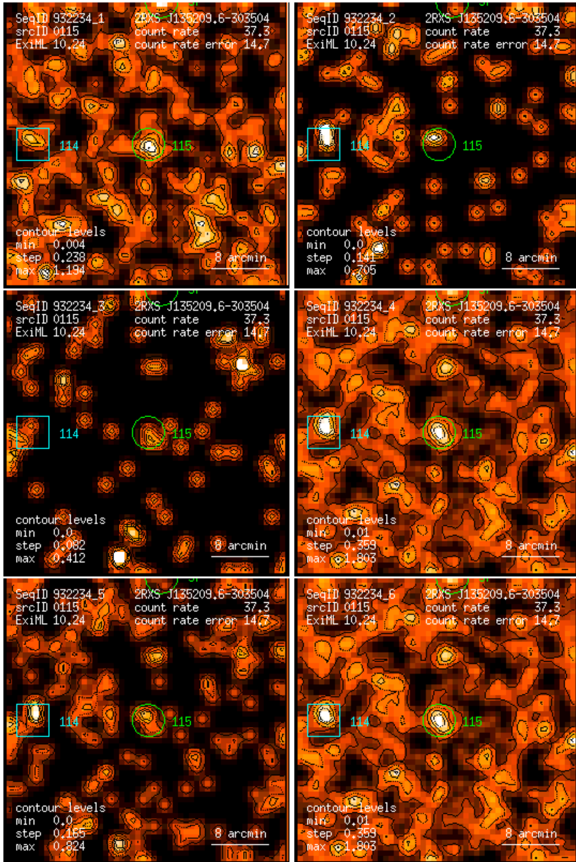
Figure 115: RASS 932234: detection 0115: band rate images, Gaussian filter: (1) PSPC channels 11 – 41, (2) 52 – 90, (3) 91 – 201, (4) 11 – 235, (5) 52 – 201, (6) 11 – 201. Broad band rates in counts/ks. Band rate contour levels in counts/ks/arcmin 2 .
