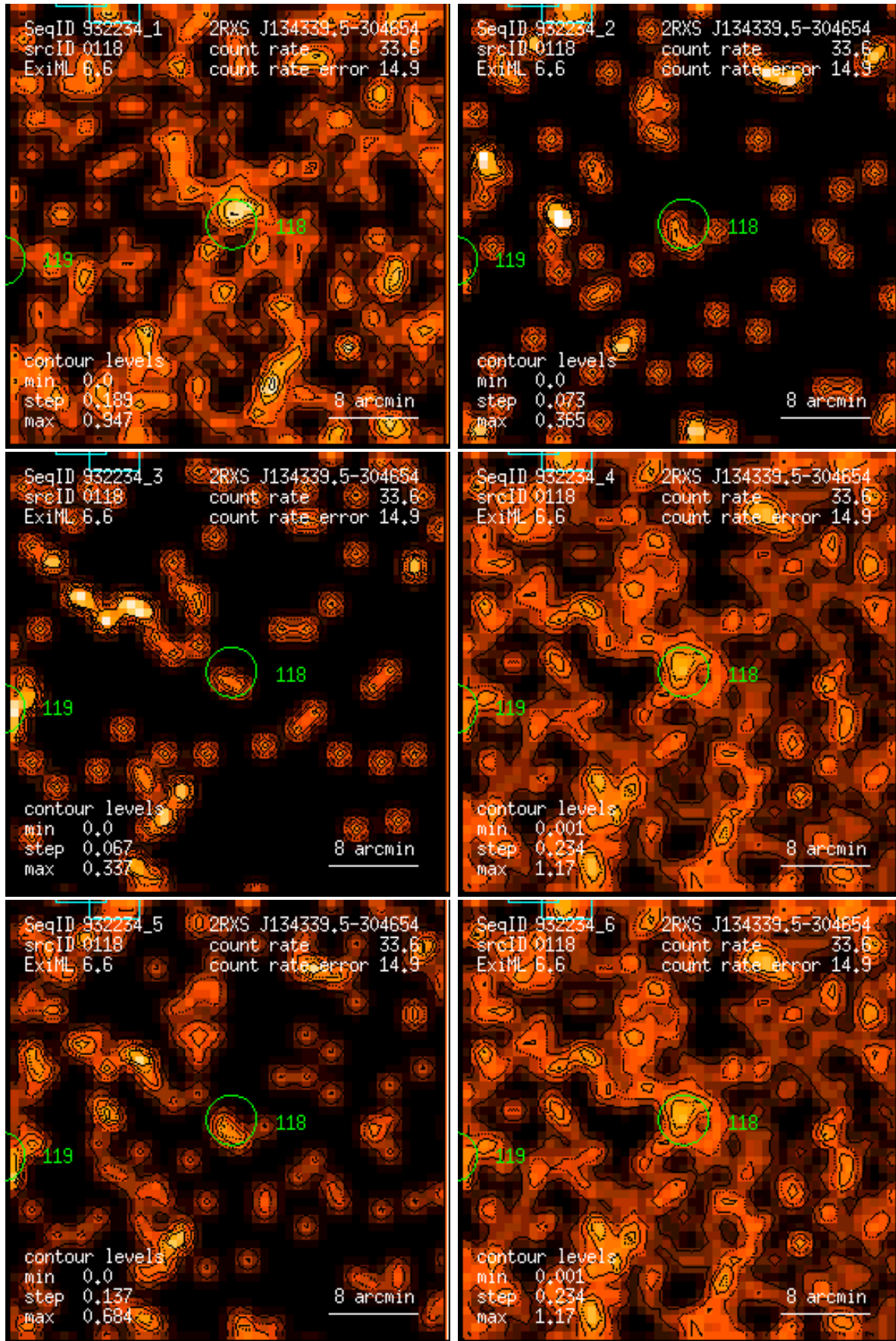
Figure 118: RASS 932234: detection 0118: band rate images, Gaussian filter: (1) PSPC channels 11 – 41, (2) 52 – 90, (3) 91 – 201, (4) 11 – 235, (5) 52 – 201, (6) 11 – 201. Broad band rates in counts/ks. Band rate contour levels in counts/ks/arcmin 2 .
