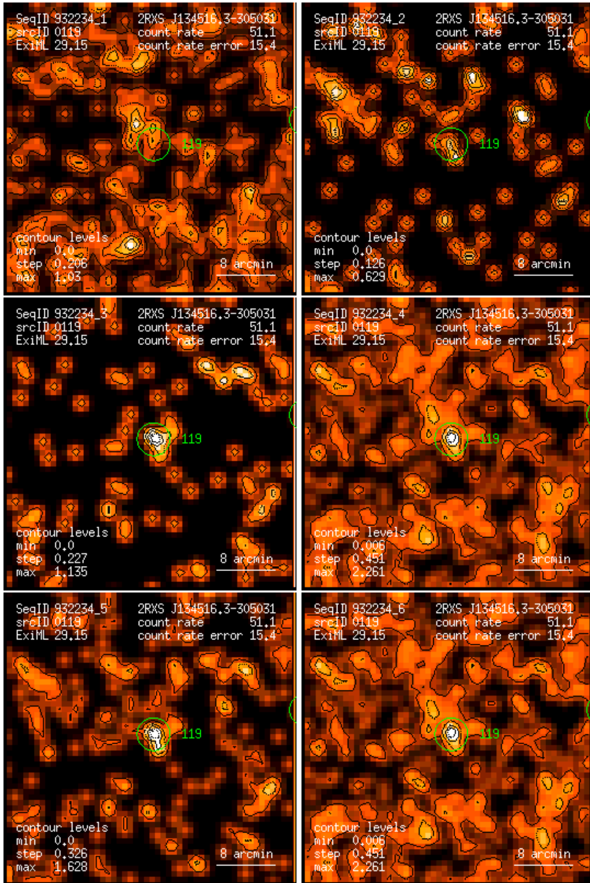
Figure 119: RASS 932234: detection 0119: band rate images, Gaussian filter: (1) PSPC channels 11 – 41, (2) 52 – 90, (3) 91 – 201, (4) 11 – 235, (5) 52 – 201, (6) 11 – 201. Broad band rates in counts/ks. Band rate contour levels in counts/ks/arcmin 2 .
