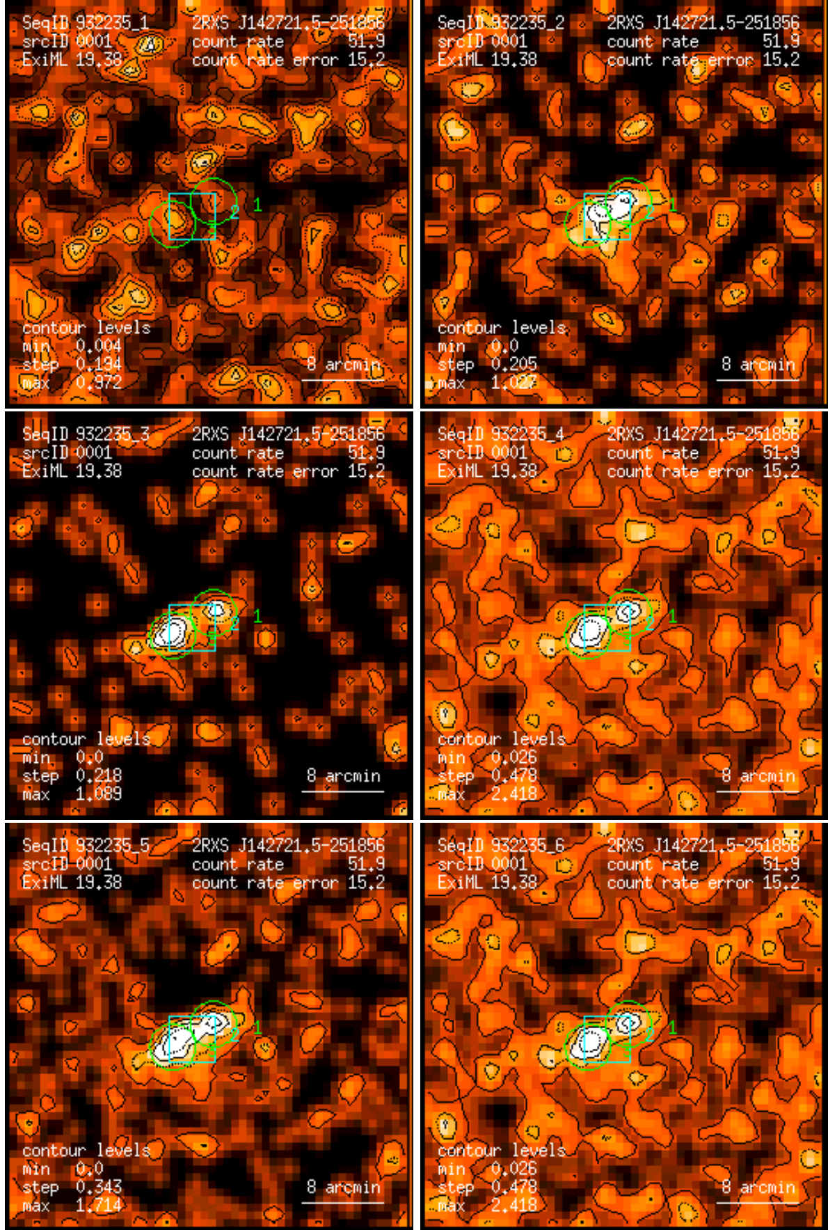
Figure 1: RASS 932235: detection 0001: band rate images, Gaussian filter: (1) PSPC channels 11 – 41, (2) 52 – 90, (3) 91 – 201, (4) 11 – 235, (5) 52 – 201, (6) 11 – 201. Broad band rates in counts/ks. Band rate contour levels in counts/ks/arcmin 2 .
