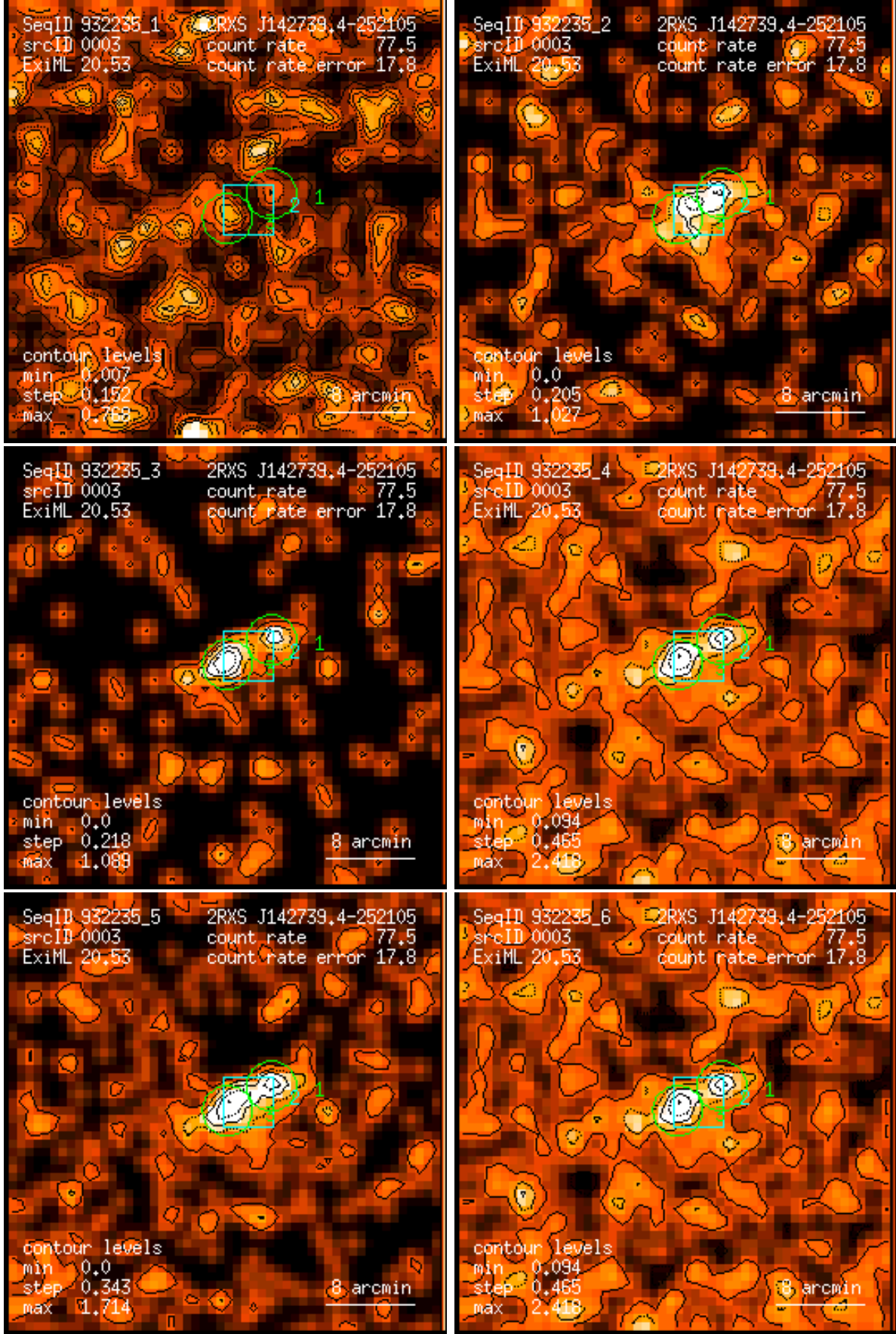
Figure 3: RASS 932235: detection 0003: band rate images, Gaussian filter: (1) PSPC channels 11 – 41, (2) 52 – 90, (3) 91 – 201, (4) 11 – 235, (5) 52 – 201, (6) 11 – 201. Broad band rates in counts/ks. Band rate contour levels in counts/ks/arcmin 2 .
