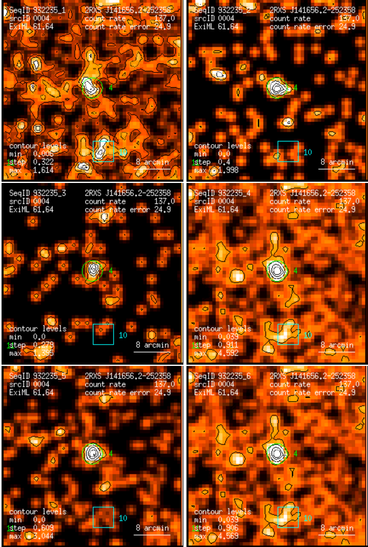
Figure 4: RASS 932235: detection 0004: band rate images, Gaussian filter: (1) PSPC channels 11 – 41, (2) 52 – 90, (3) 91 – 201, (4) 11 – 235, (5) 52 – 201, (6) 11 – 201. Broad band rates in counts/ks. Band rate contour levels in counts/ks/arcmin 2 .
