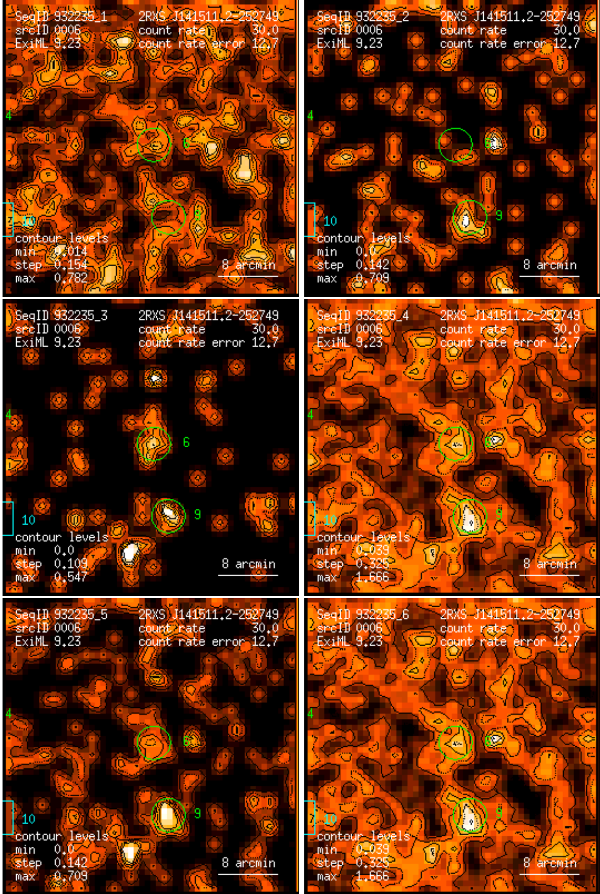
Figure 6: RASS 932235: detection 0006: band rate images, Gaussian filter: (1) PSPC channels 11 – 41, (2) 52 – 90, (3) 91 – 201, (4) 11 – 235, (5) 52 – 201, (6) 11 – 201. Broad band rates in counts/ks. Band rate contour levels in counts/ks/arcmin 2 .
