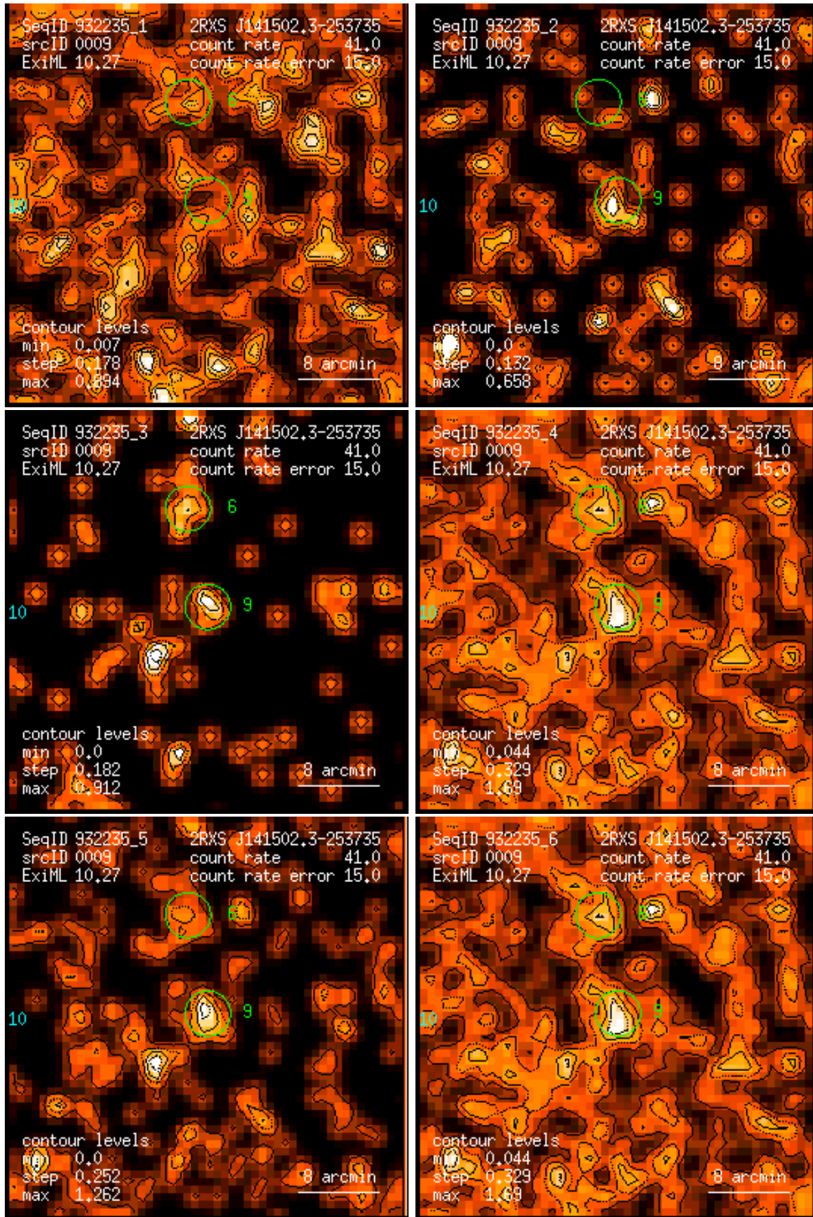
Figure 9: RASS 932235: detection 0009: band rate images, Gaussian filter: (1) PSPC channels 11 – 41, (2) 52 – 90, (3) 91 – 201, (4) 11 – 235, (5) 52 – 201, (6) 11 – 201. Broad band rates in counts/ks. Band rate contour levels in counts/ks/arcmin 2 .
