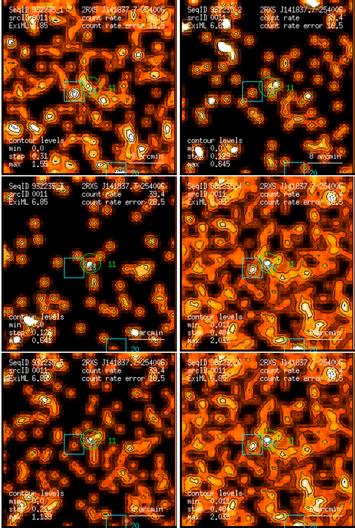
Figure 11: RASS 932235: detection 0011: band rate images, Gaussian filter: (1) PSPC channels 11 – 41, (2) 52 – 90, (3) 91 – 201, (4) 11 – 235, (5) 52 – 201, (6) 11 – 201. Broad band rates in counts/ks. Band rate contour levels in counts/ks/arcmin 2 .
