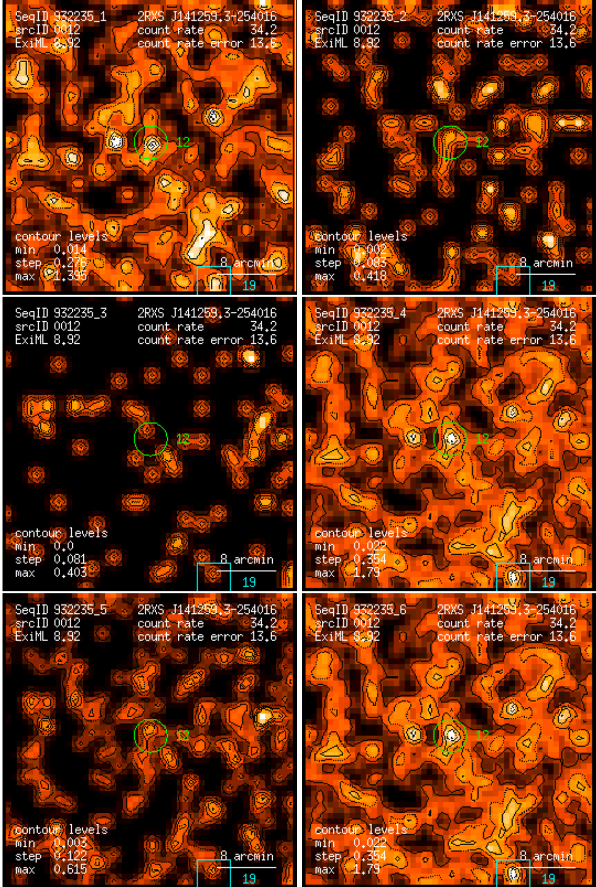
Figure 12: RASS 932235: detection 0012: band rate images, Gaussian filter: (1) PSPC channels 11 – 41, (2) 52 – 90, (3) 91 – 201, (4) 11 – 235, (5) 52 – 201, (6) 11 – 201. Broad band rates in counts/ks. Band rate contour levels in counts/ks/arcmin 2 .
