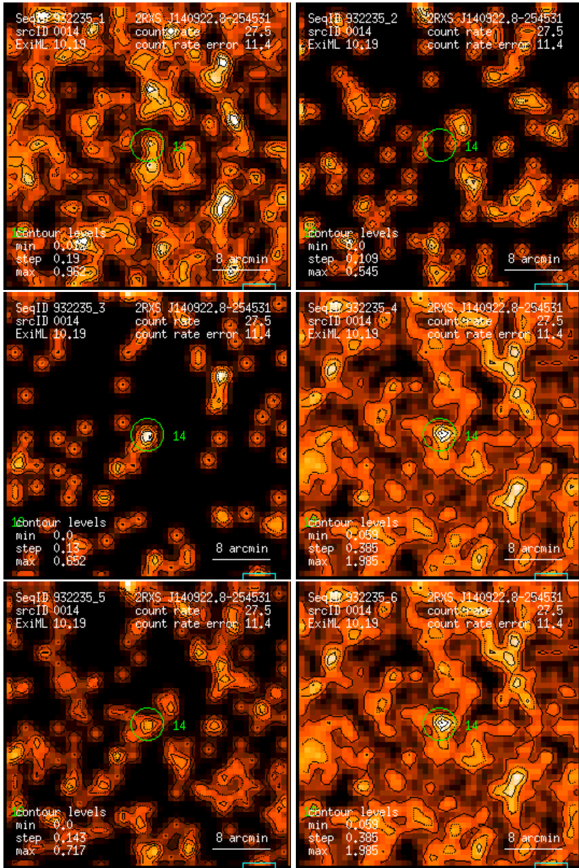
Figure 14: RASS 932235: detection 0014: band rate images, Gaussian filter: (1) PSPC channels 11 – 41, (2) 52 – 90, (3) 91 – 201, (4) 11 – 235, (5) 52 – 201, (6) 11 – 201. Broad band rates in counts/ks. Band rate contour levels in counts/ks/arcmin 2 .
