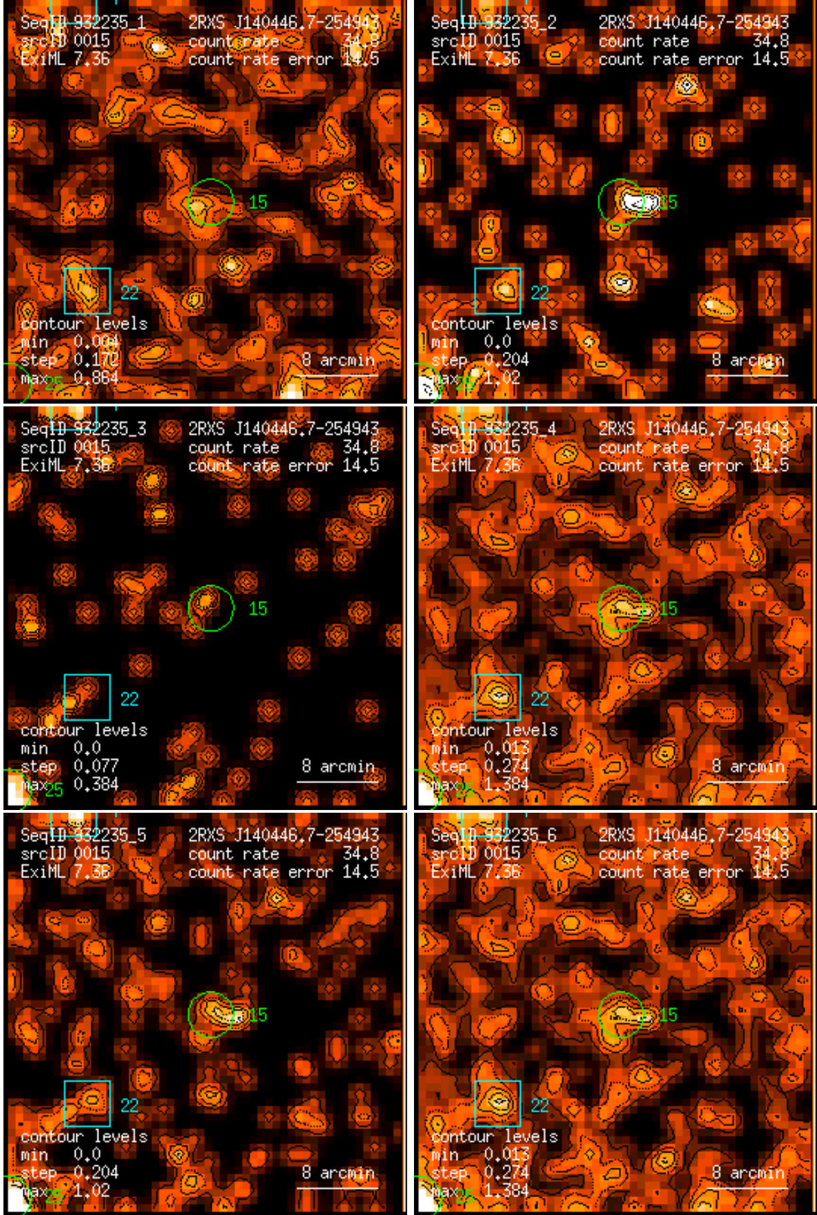
Figure 15: RASS 932235: detection 0015: band rate images, Gaussian filter: (1) PSPC channels 11 – 41, (2) 52 – 90, (3) 91 – 201, (4) 11 – 235, (5) 52 – 201, (6) 11 – 201. Broad band rates in counts/ks. Band rate contour levels in counts/ks/arcmin 2 .
