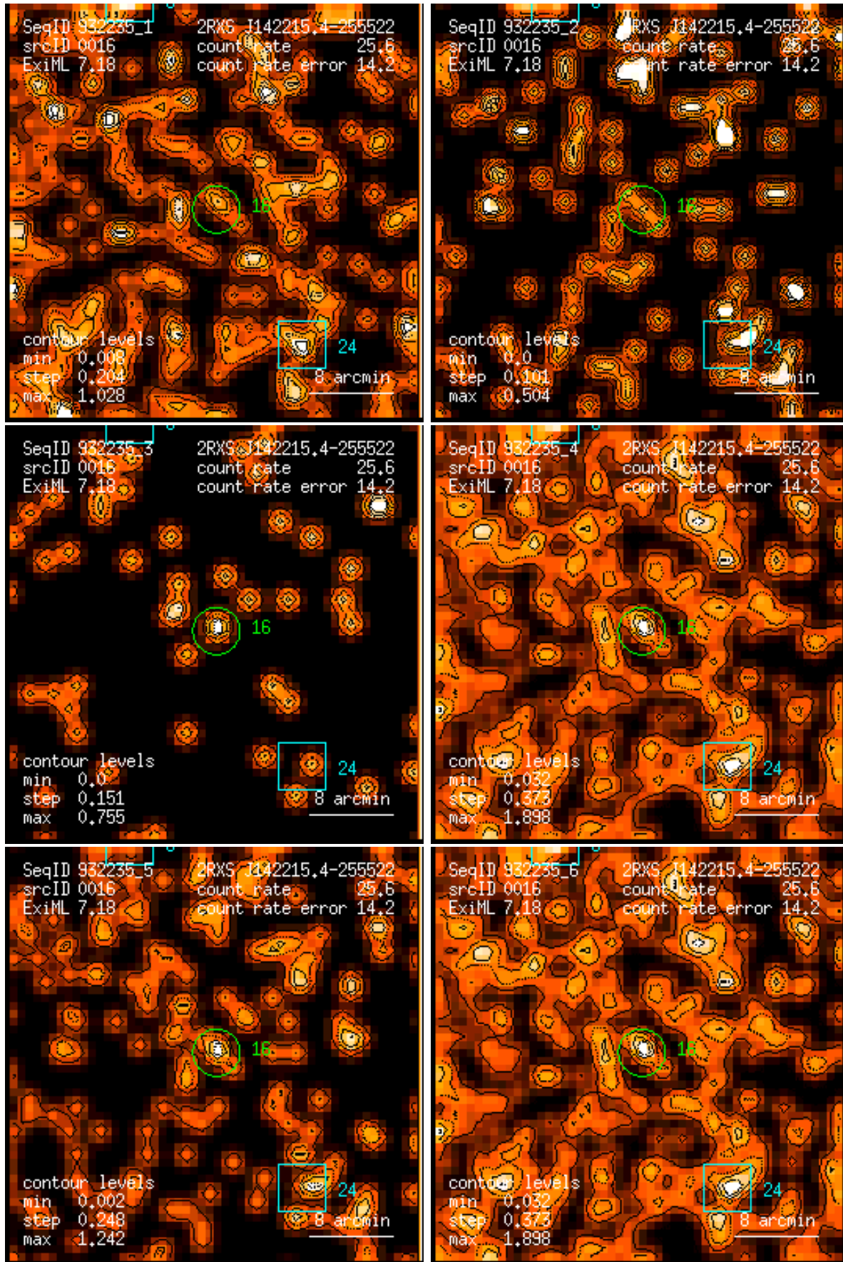
Figure 16: RASS 932235: detection 0016: band rate images, Gaussian filter: (1) PSPC channels 11 – 41, (2) 52 – 90, (3) 91 – 201, (4) 11 – 235, (5) 52 – 201, (6) 11 – 201. Broad band rates in counts/ks. Band rate contour levels in counts/ks/arcmin 2 .
