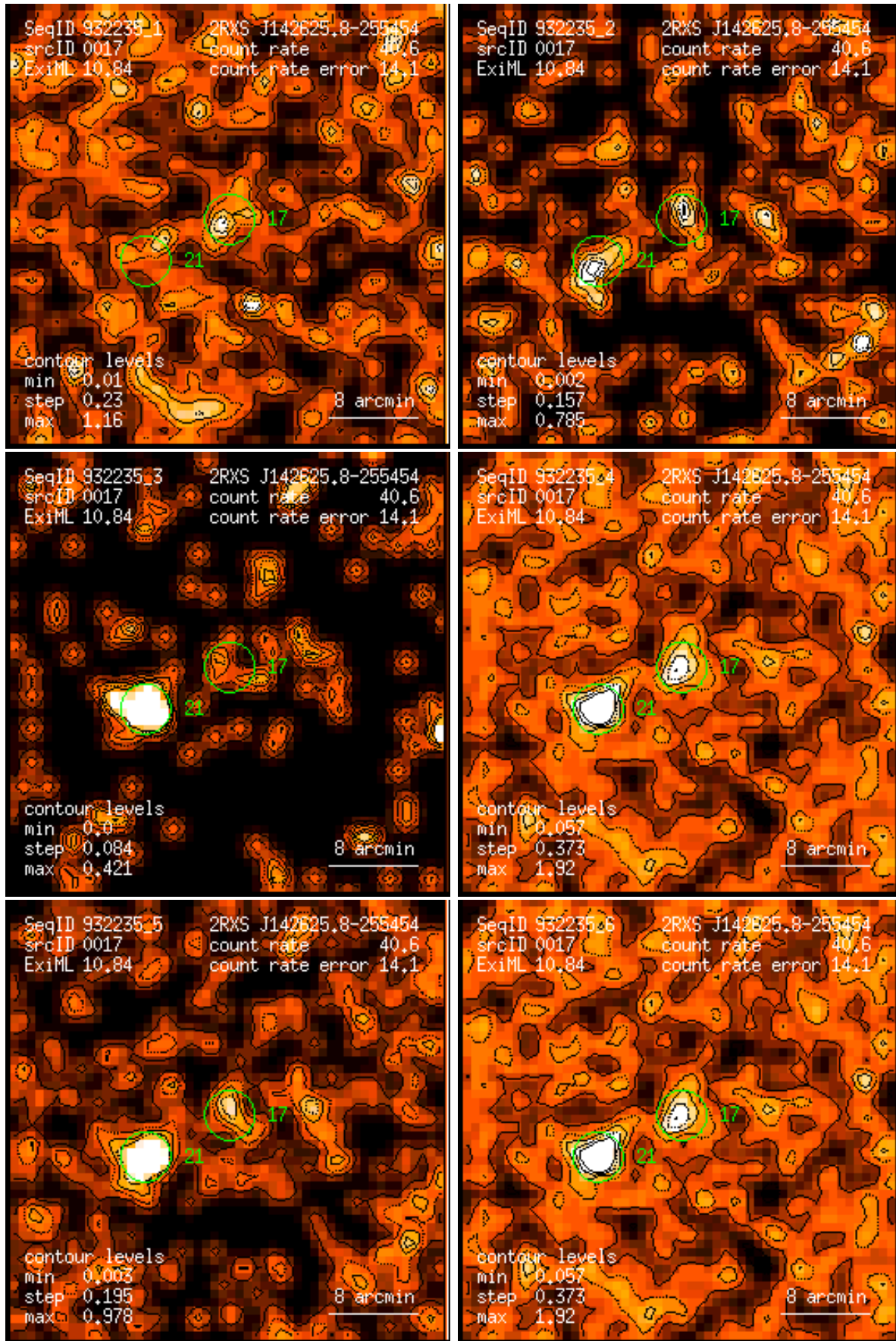
Figure 17: RASS 932235: detection 0017: band rate images, Gaussian filter: (1) PSPC channels 11 – 41, (2) 52 – 90, (3) 91 – 201, (4) 11 – 235, (5) 52 – 201, (6) 11 – 201. Broad band rates in counts/ks. Band rate contour levels in counts/ks/arcmin 2 .
