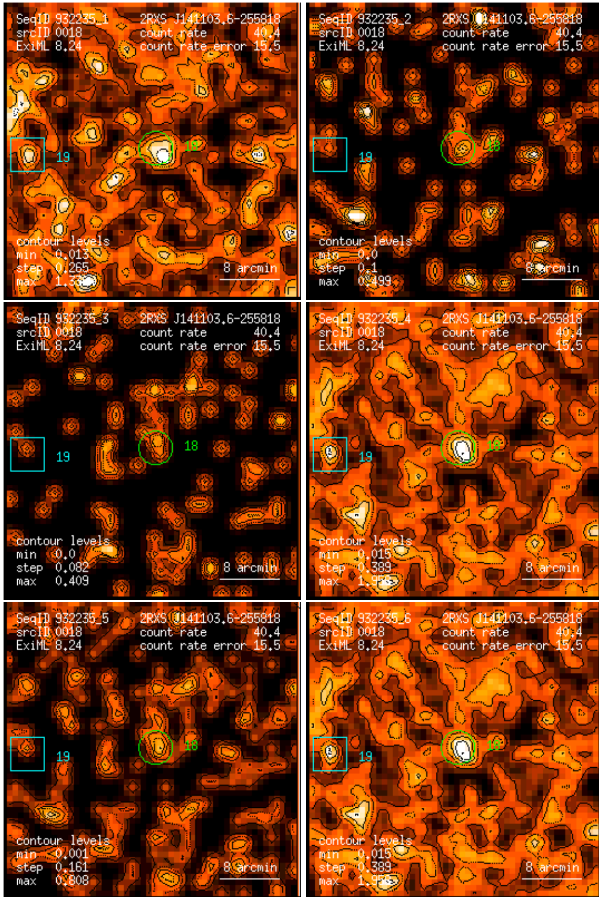
Figure 18: RASS 932235: detection 0018: band rate images, Gaussian filter: (1) PSPC channels 11 – 41, (2) 52 – 90, (3) 91 – 201, (4) 11 – 235, (5) 52 – 201, (6) 11 – 201. Broad band rates in counts/ks. Band rate contour levels in counts/ks/arcmin 2 .
